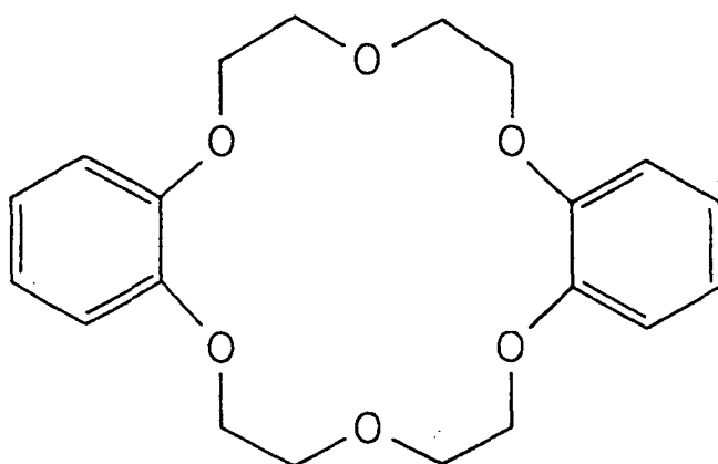
DIBENZOYL-18-CROWN-6
