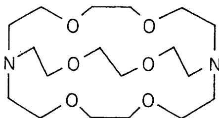
CRYPTAND [2.2.2]
