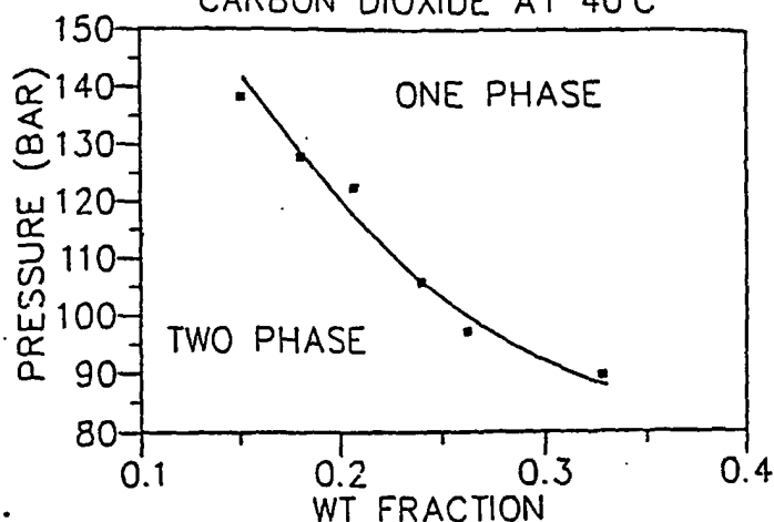
POLY(CHLOROTRIFLUOROETHYLENE) IN CARBON DIOXIDE AT 40°C
