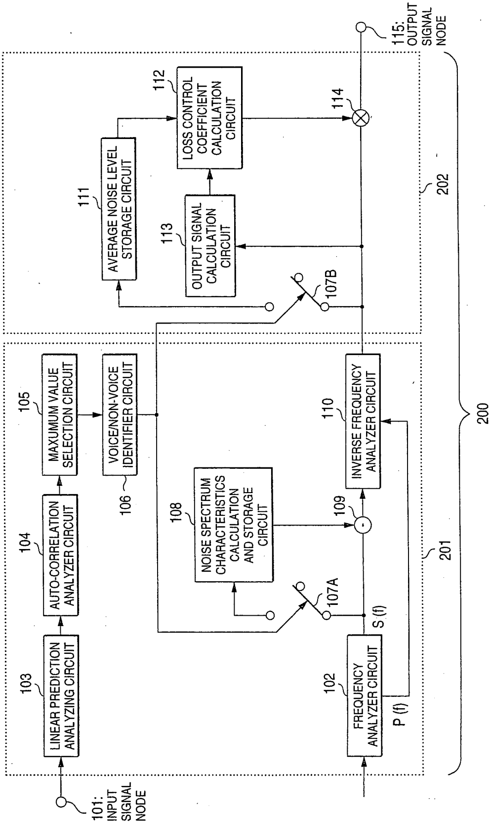
FIG. 1 PRIOR ART
