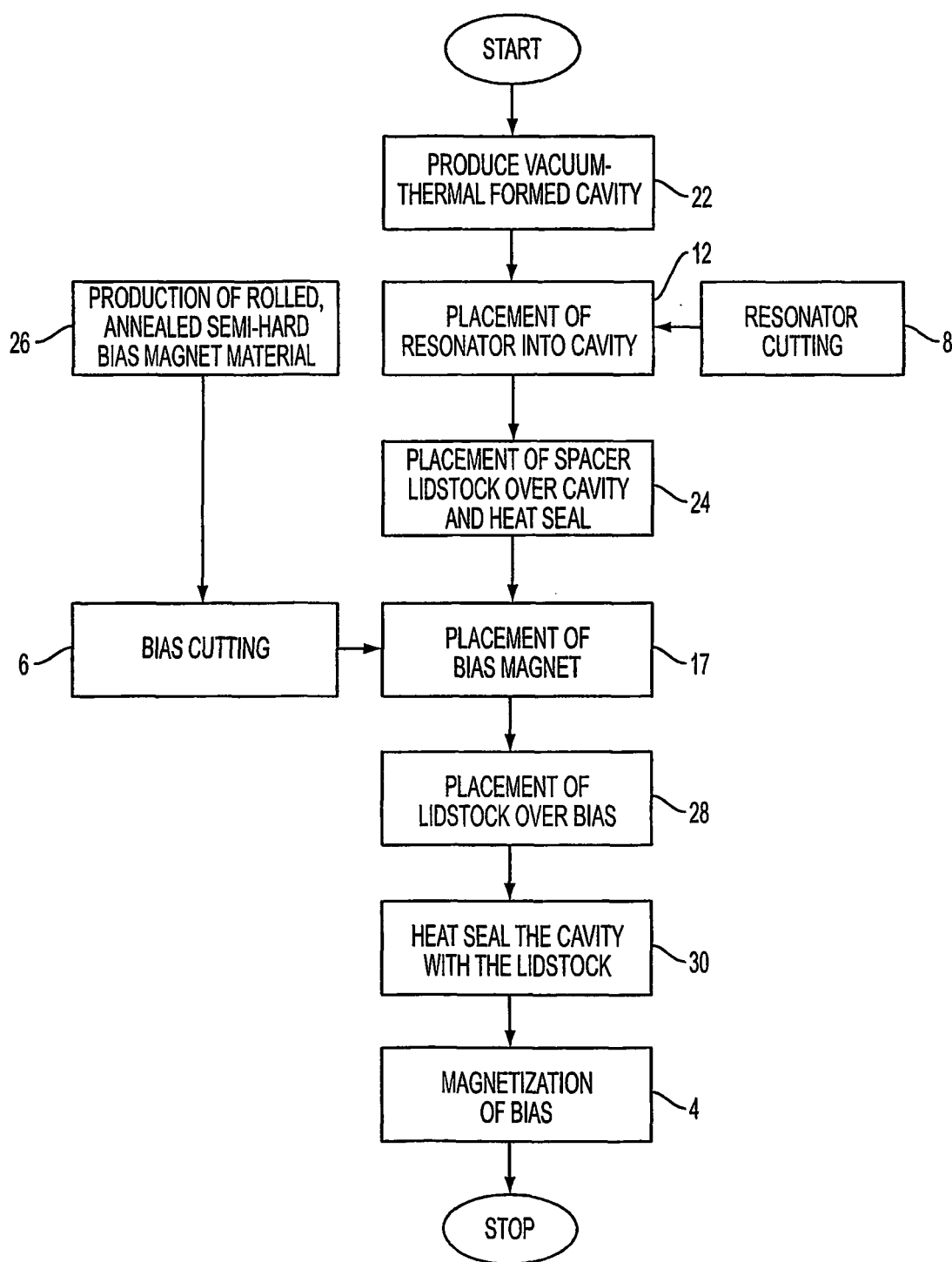
FIG. 2 (PRIOR ART)
