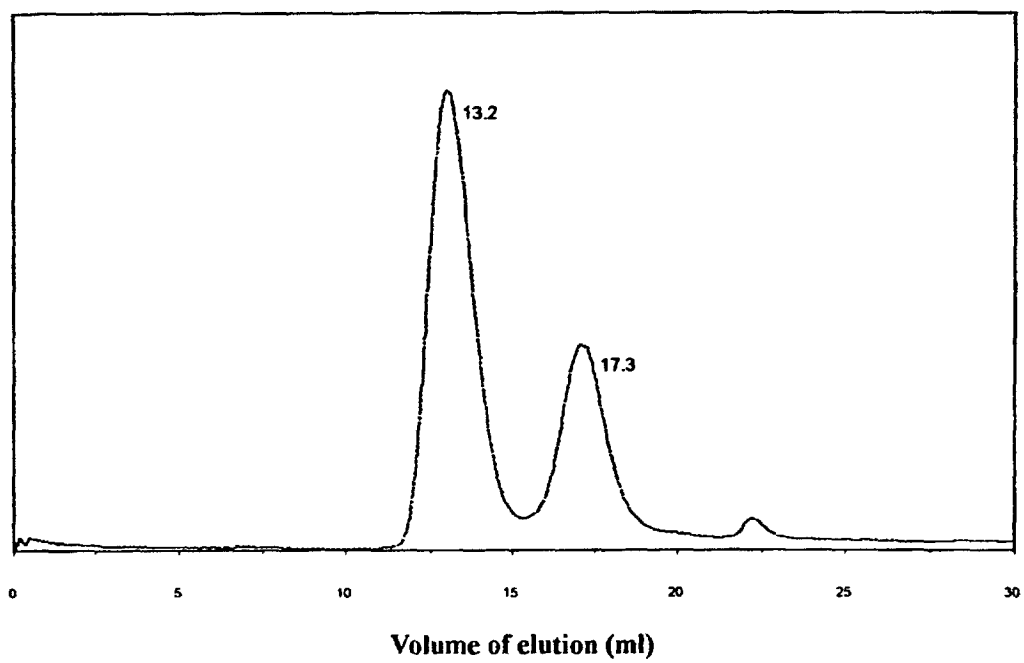
Fig2 Elution profile on Superdex-75 column
