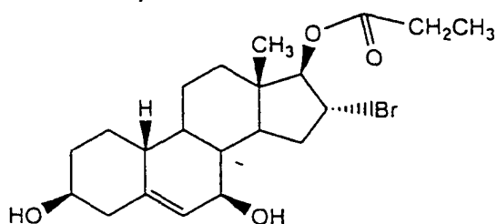
group 9-2 compound 1.2.1.9.
