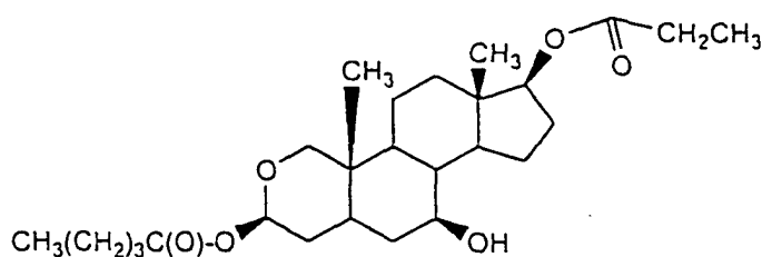
group 28-11-1 compound
