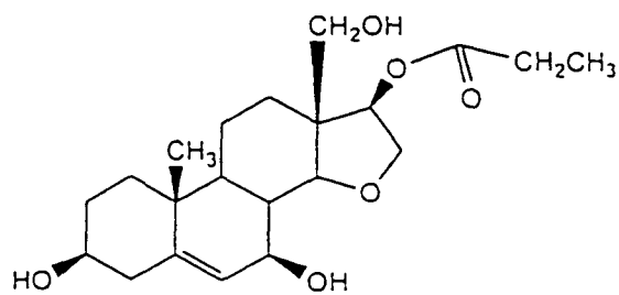
group 26-8-2 compound 1.2.5.9.
