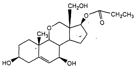
group 27-8-2 compound 1.2.5.9.
