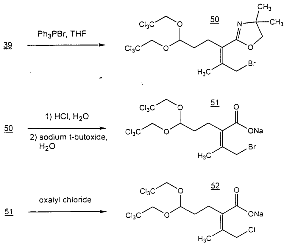
Scheme 12D
