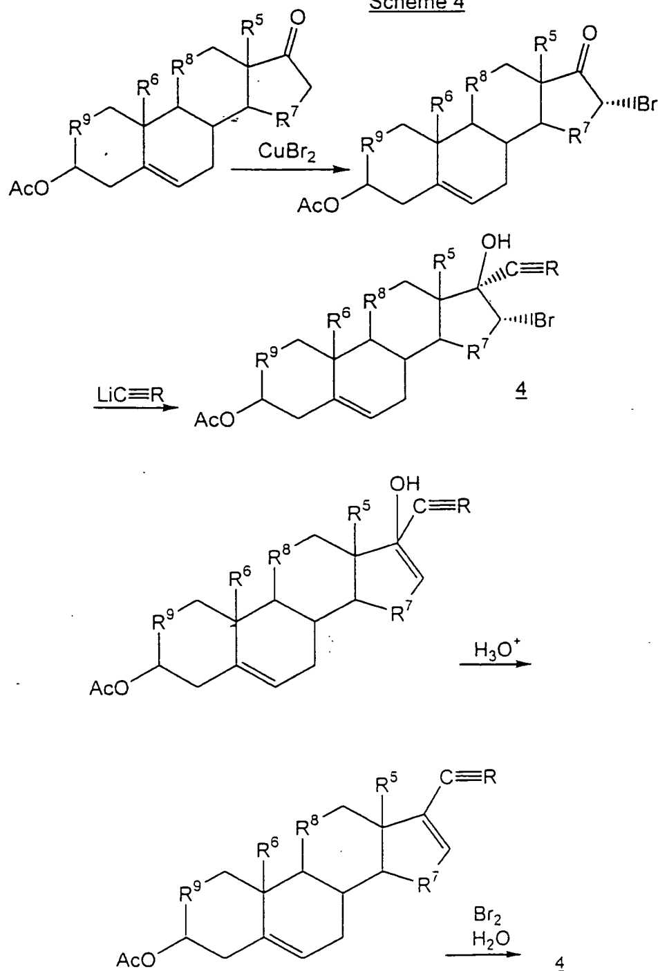
Scheme 4
