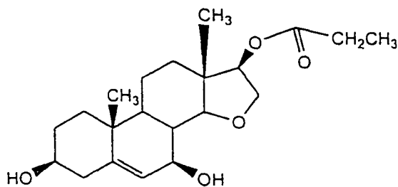
group 26-2 compound 1.2.5.9.
