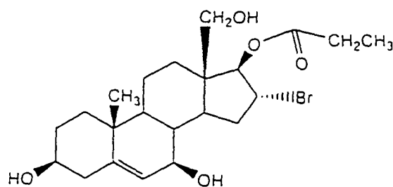
group 8-2 compound 1.2.1.9.
