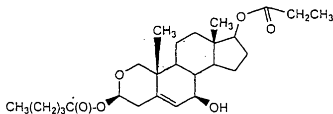
group 28-11-2 compound
