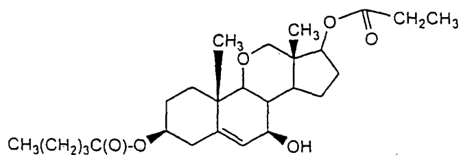
group 27-11-2 compound
