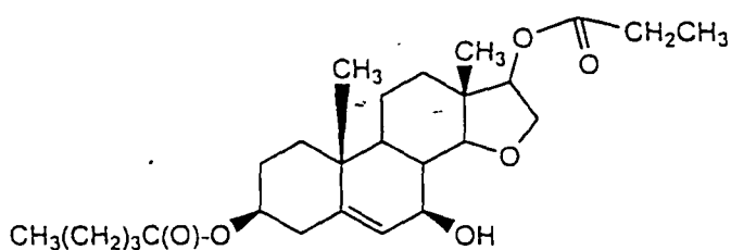
group 26-11-2 compound
