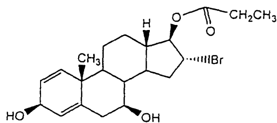
group 7-6 compound 1.2.1.9.
