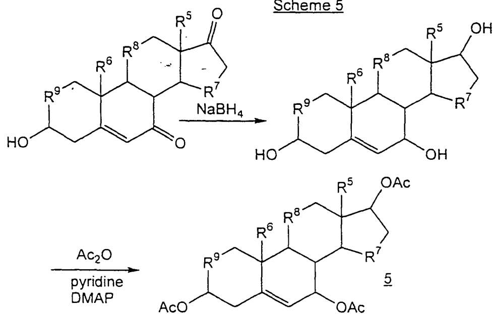
Scheme 5
