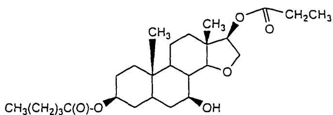
group 26-11-1 compound
