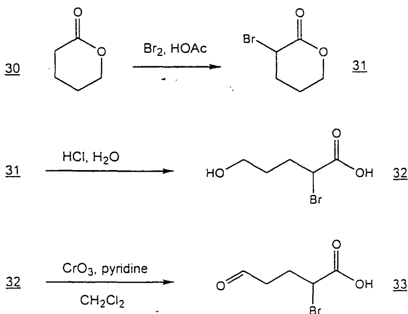
Scheme 12A
