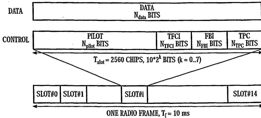
B. FRAME STRUCTURE OF UPLINK
