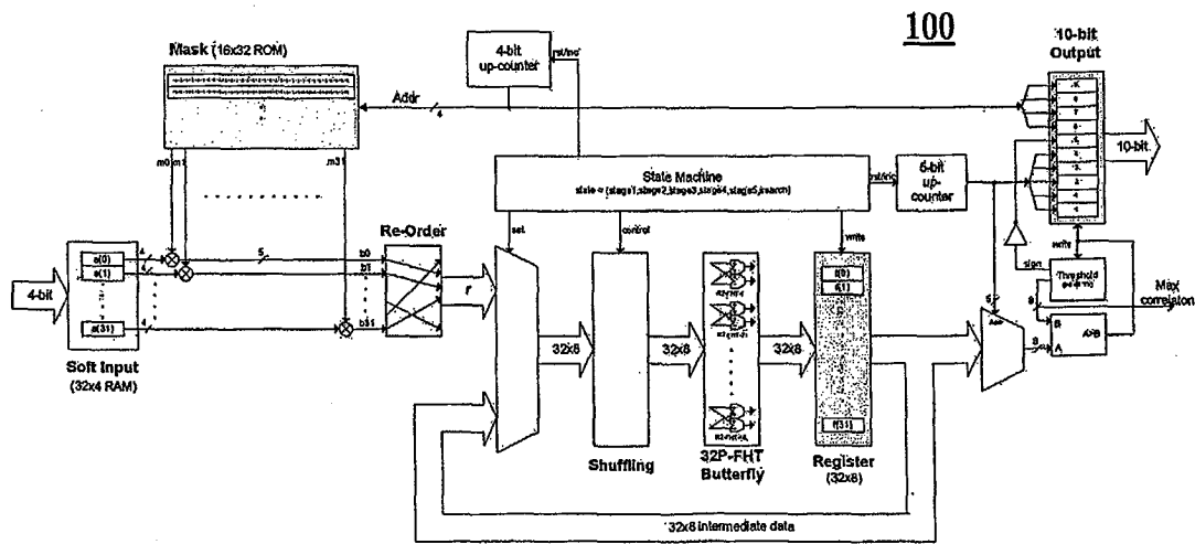
FIG. 4 (PRIOR ART)
