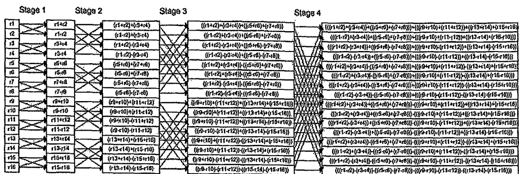
FIG. 5 (PRIOR ART)
