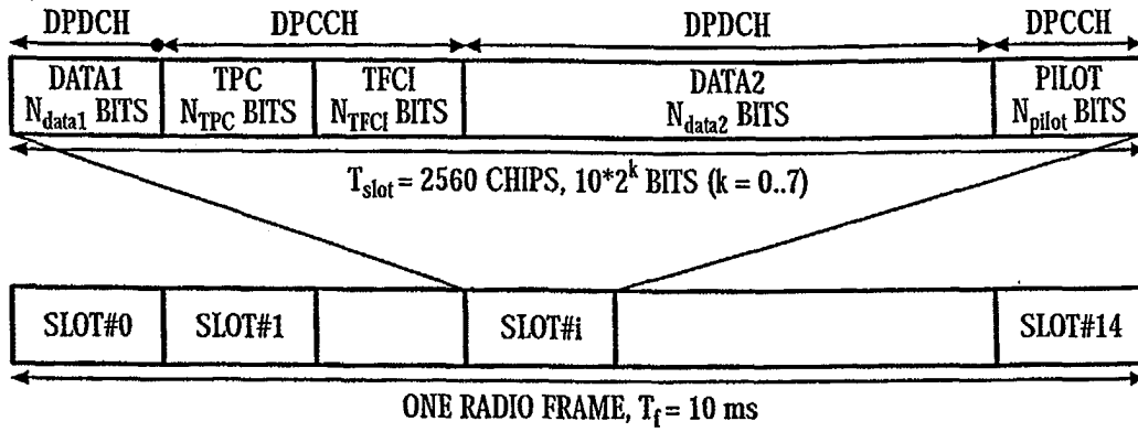
A. FRAME STRUCTURE OF DOWNLINK
