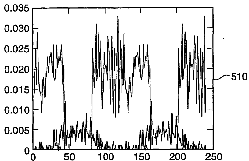
FIG. 5a 1.0 Torr
