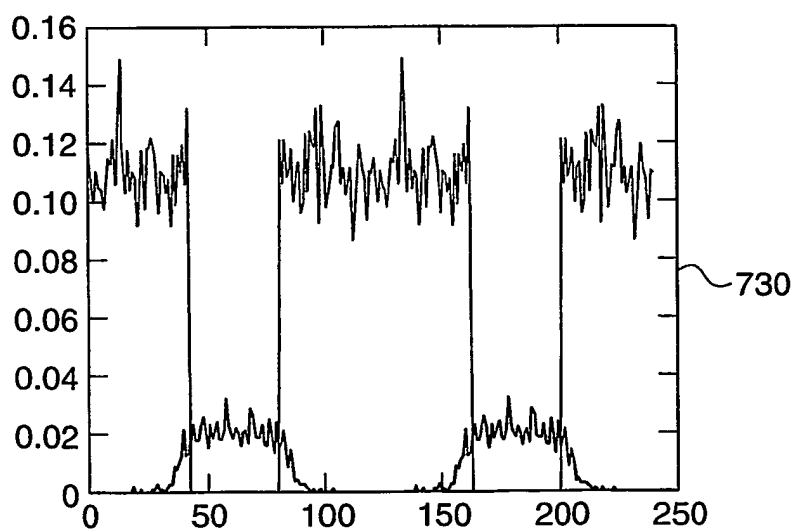
FIG. 7c t = 54 \mu\text{m}
