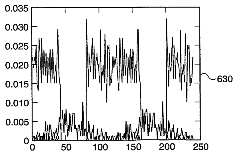
FIG. 6c s = 20 \mu\text{m}
