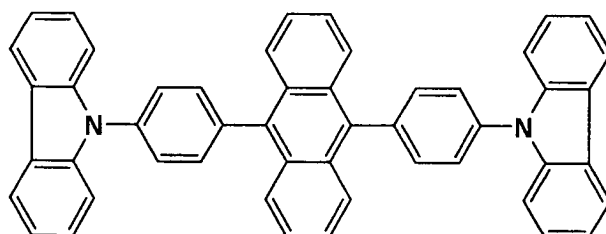
Comparative compound 5
