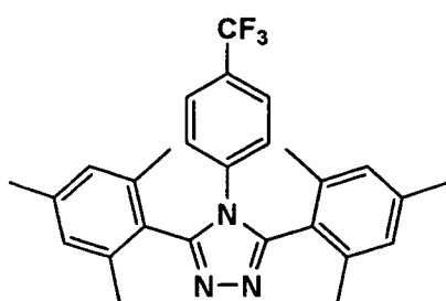
C1-1
