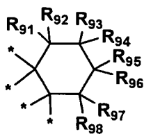
formula (j)
