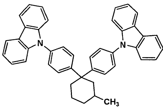
4-5
