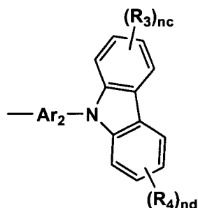
Formula 4
