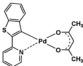
Pd-3
