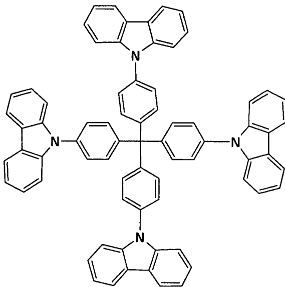
Comparative compound 11
