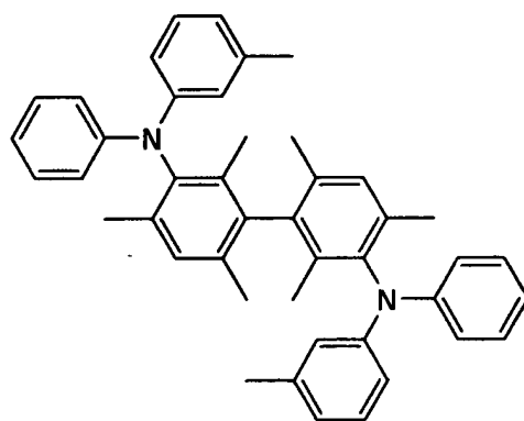
C-17
