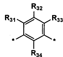
formula (c)
