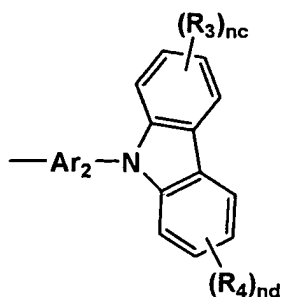
Formula 4
