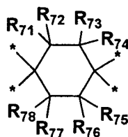
formula (h)
