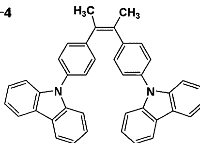
2-5
