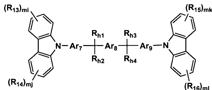
Formula H3
