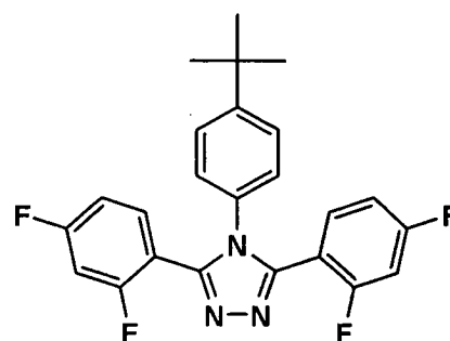
B1-4
