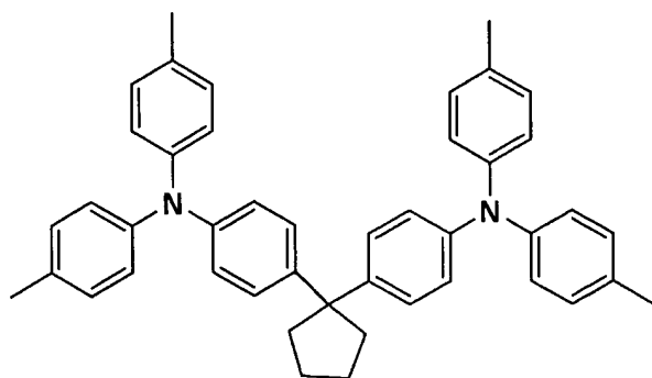
C-15
