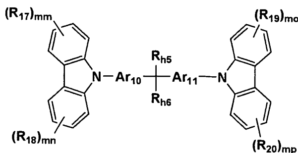
Formula H4
