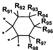
formula (j)
