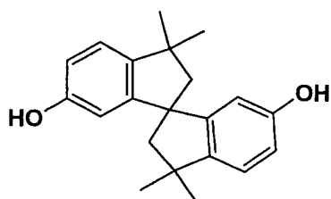
Bisphenol compound
