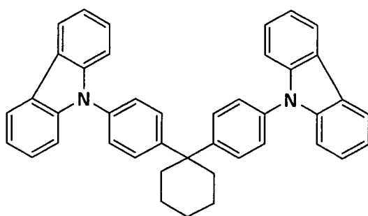
Comparative compound 2
