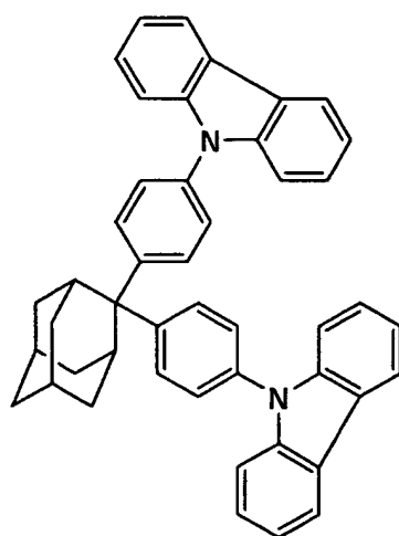
Comparative compound 8
