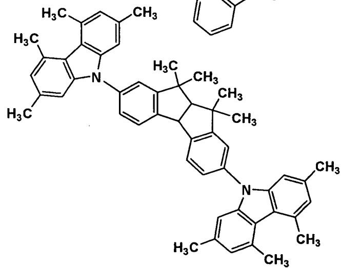
IA-14
