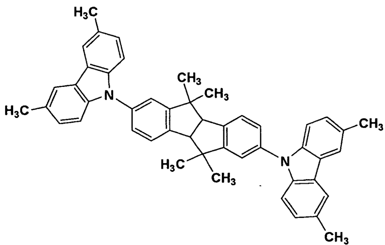
IA-11
