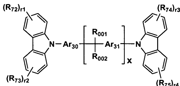
Formula K
