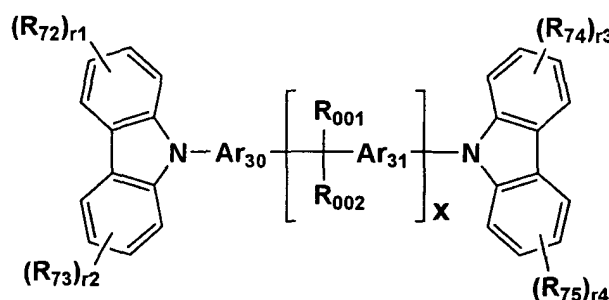
Formula K
