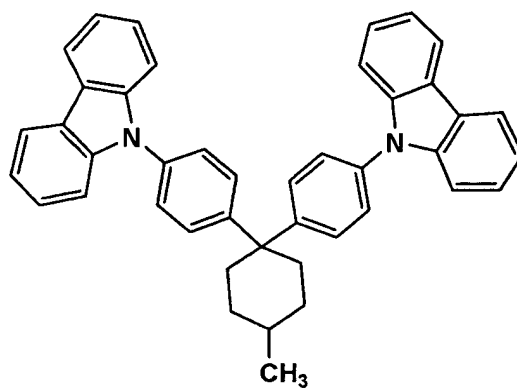
4-4
