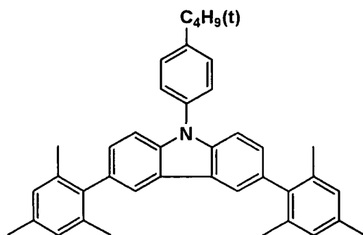
C-10
