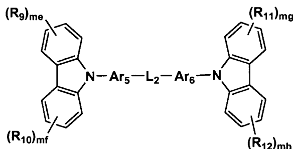
Formula H2
