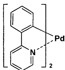
Rh-1
