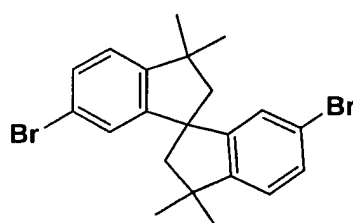
Dibromo compound
