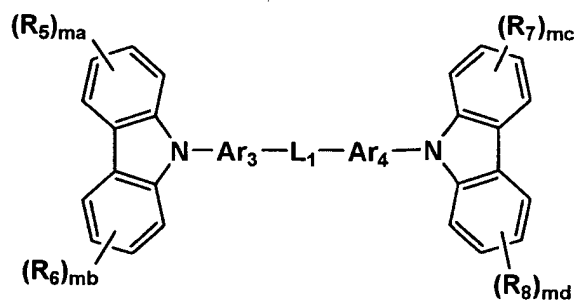
Formula H1
