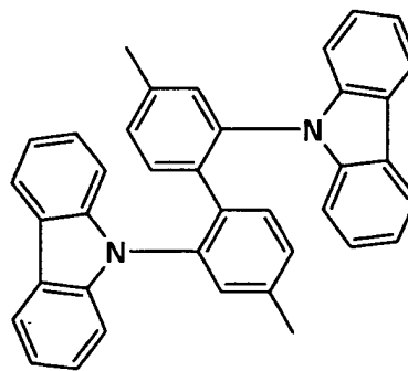
C-14
