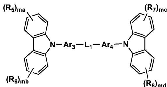
Formula H1
