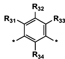
formula (c)
