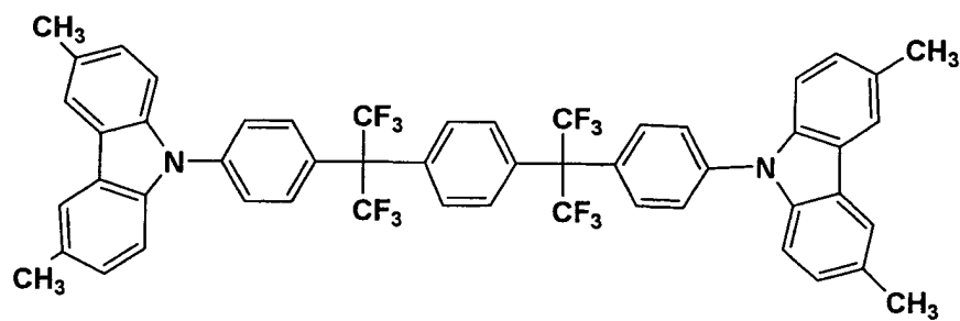
HC12
