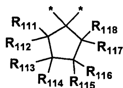
Formula (m)
