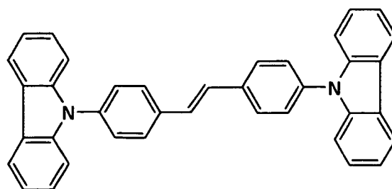
Comparative compound 6
