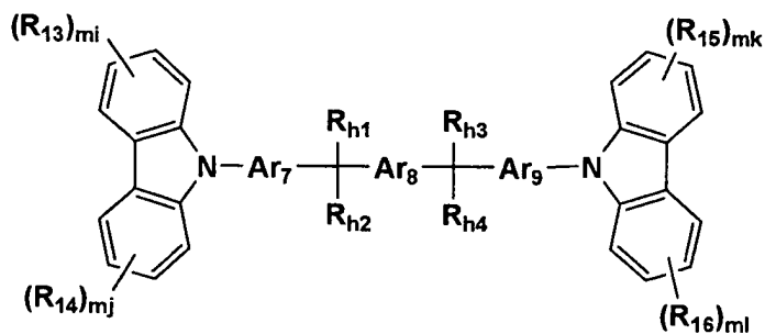
Formula H3
