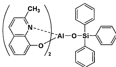
Compound A1
