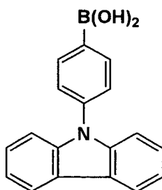
Compound B
