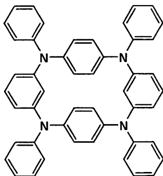
C-19
