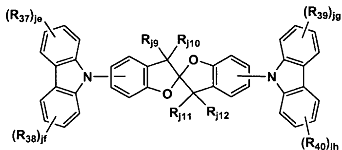
Formula J2
