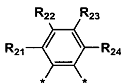
formula (b)
