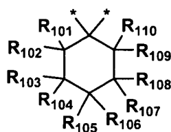
Formula (l)
