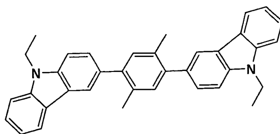
C-12
