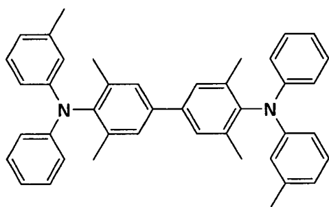
C-8
