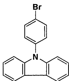
Compound A
