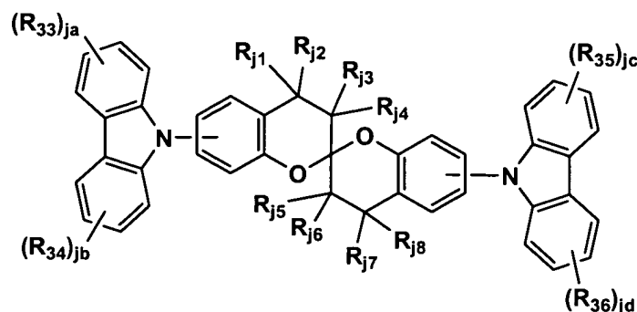
Formula J1
