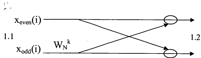
Figure 1. Butterfly, the basic computational block of FFT/IFFT
