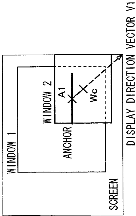
FIG. 20B FIND DISPLAY POSITION
