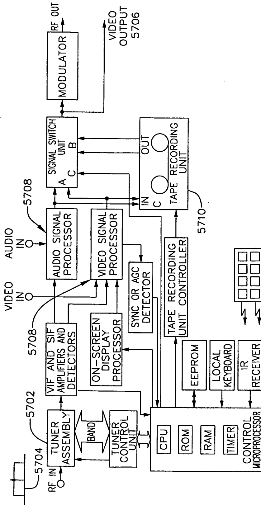
FIG. 57 VCR BLOCK DIAGRAM
