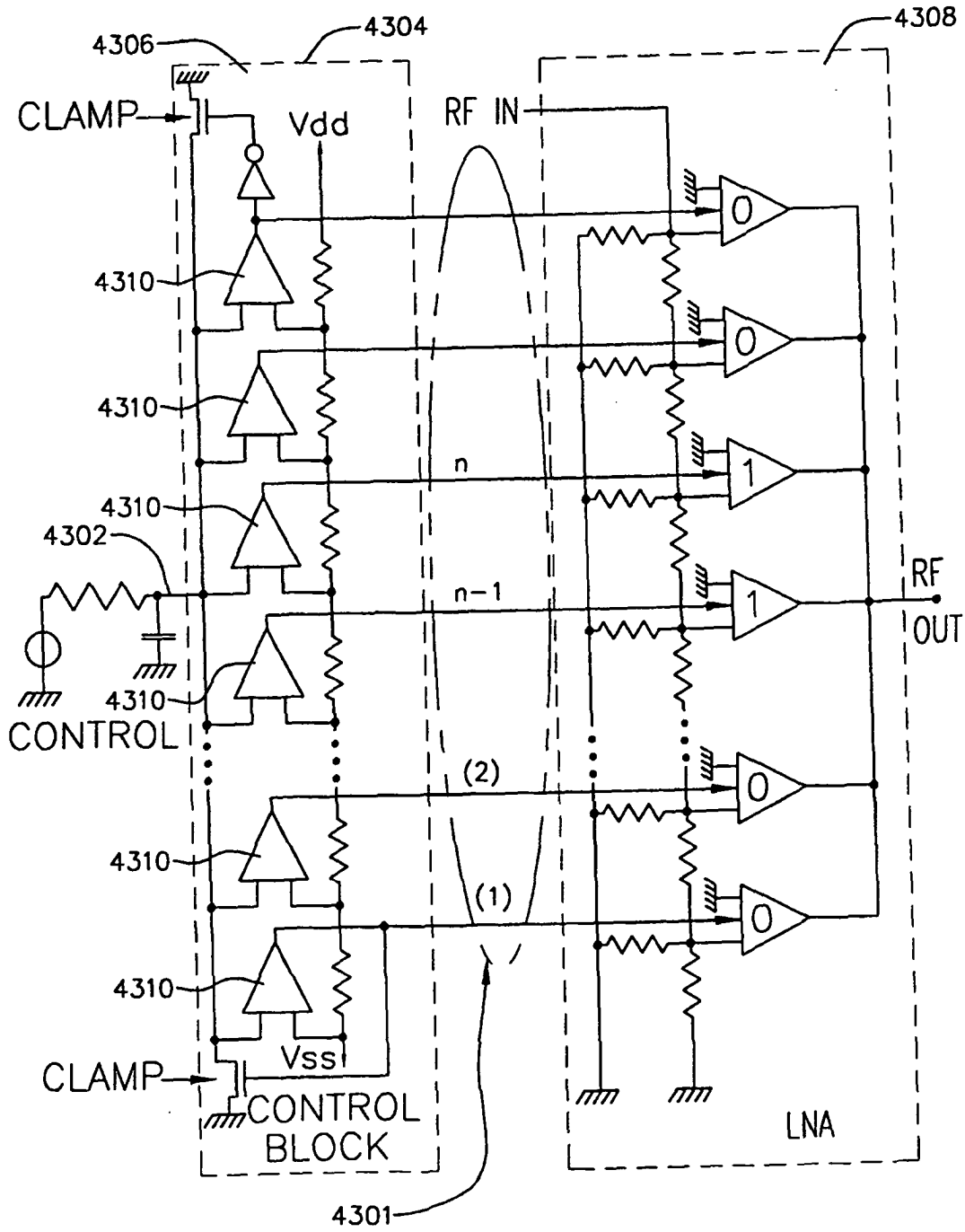
FIG. 43 CLAMPING CONTROL RANGE
