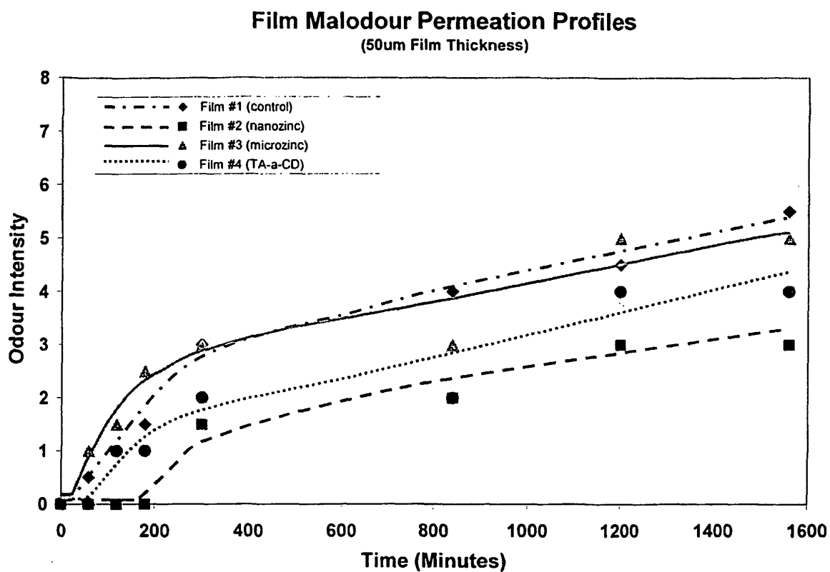
Figure 11. Closed-volume Malodour permeation profiles for Film #1, Film #2, Film #3 and Film #4 as a function of time. Permeation temperature 22°C and all film thicknesses 50 \mu\text{m} .
