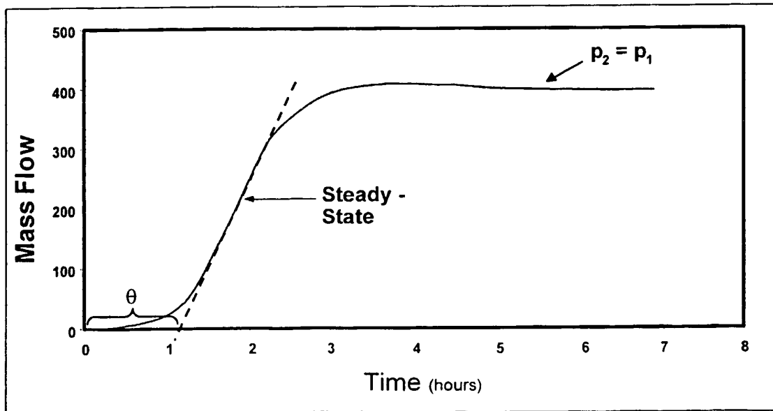
Figure 4. Typical Permeation profile with lag time \theta , steady-state and equilibrium concentration p_2 = p_1 .
