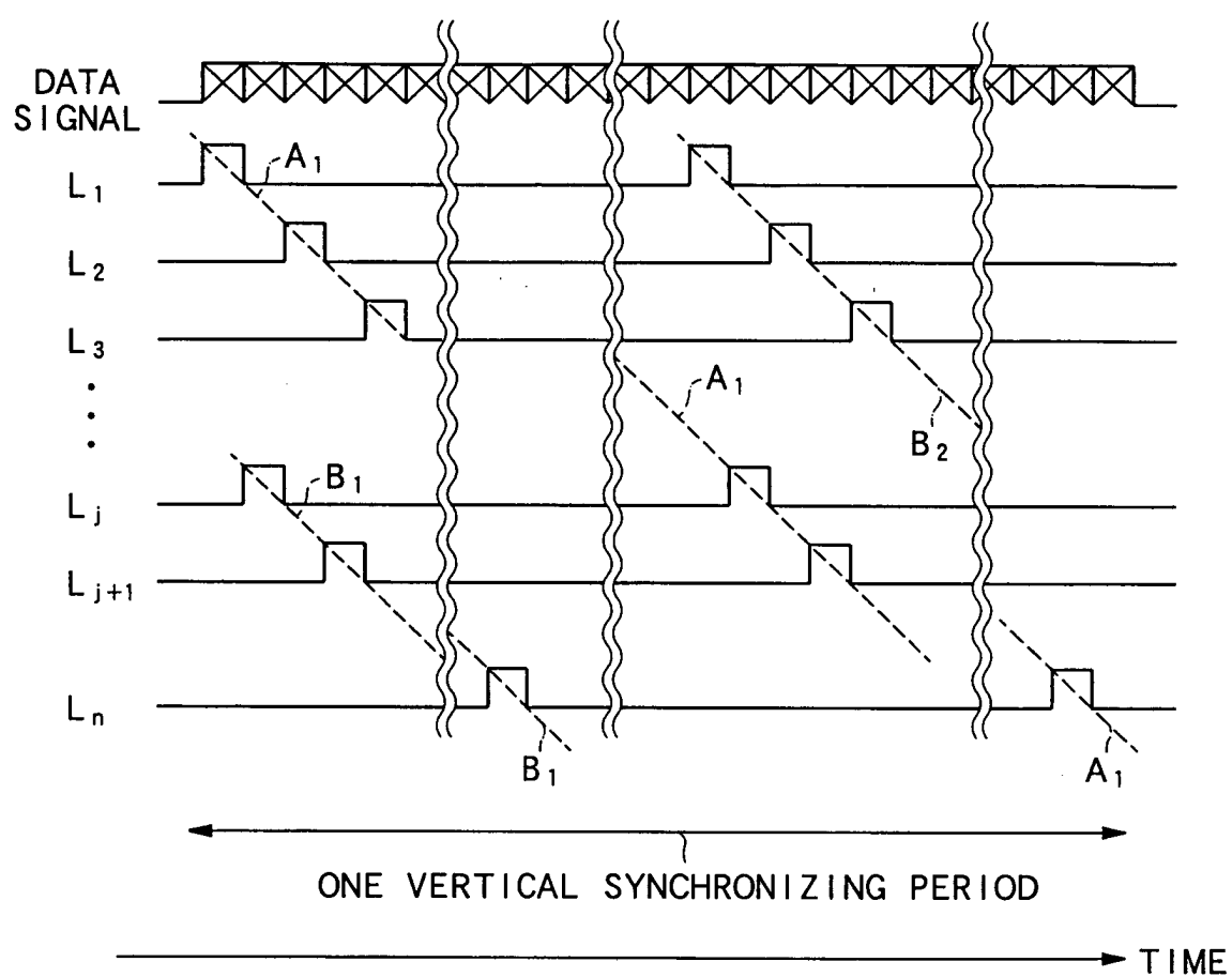
TIMING CHART (I) SHOWING A DRIVING STATE OF A DISPLAY DEVICE ACCORDING TO EMBODIMENT 2
