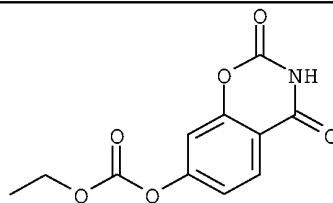
7-(ethylcarbonato)-benzo[e][1,3]oxazine-2,4-dione
