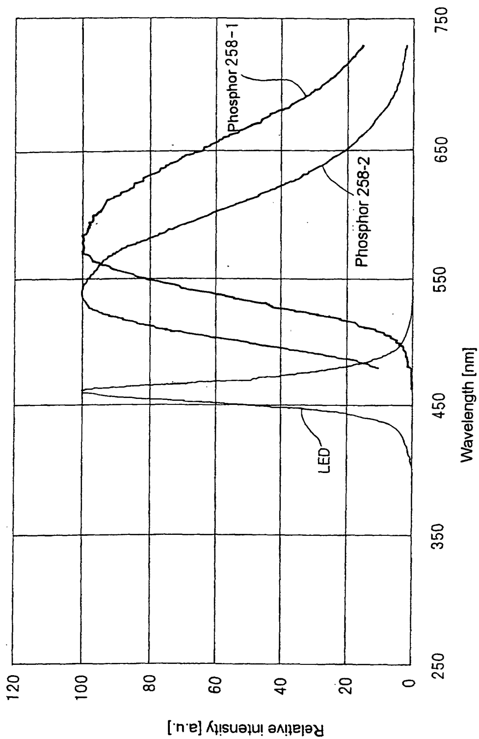
Luminescence spectra of YAG-base phosphors
