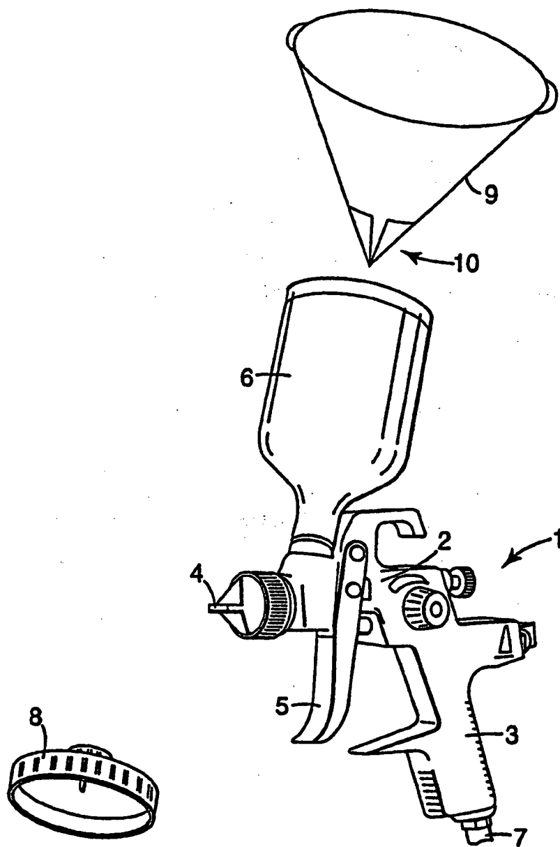
Fig. 1 PRIOR ART
