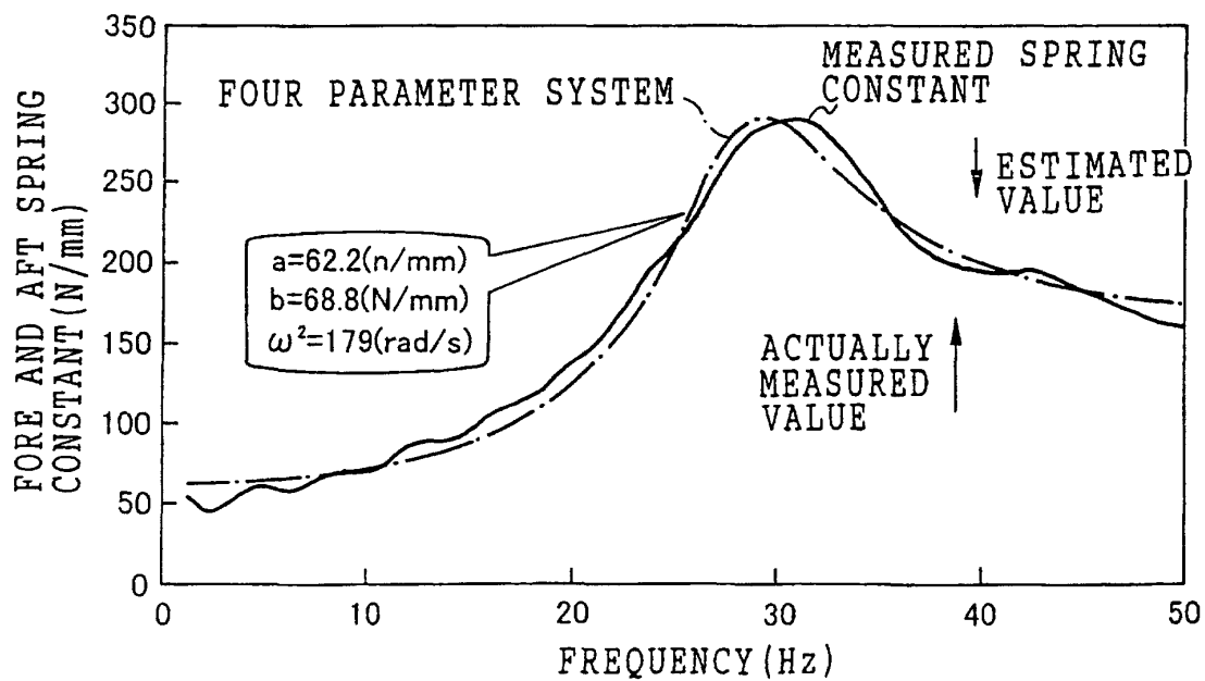
FIG. 15 DYNAMIC FORE AND AFT SPRING CONSTANT
