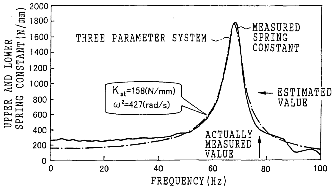
FIG. 14 DYNAMIC UPPER SPRING CONSTANT
