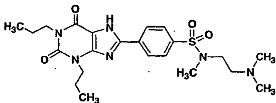
8-[4-[[[Methyl-(2-dimethylaminoethyl)-amino]sulfonyl]phenyl]-1,3-Dipropylxanthine
