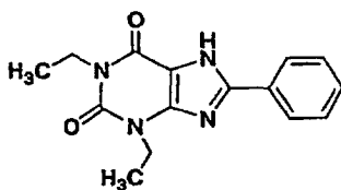
1,3-Diethyl-8-phenylxanthine
