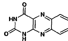
Alloxazine
