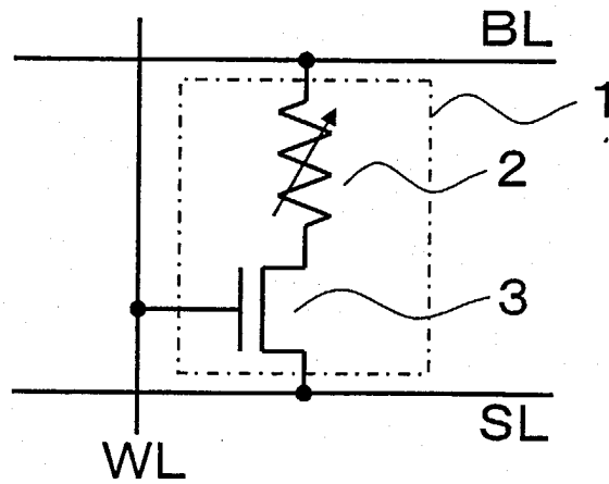
FIG.6 PRIOR ART
