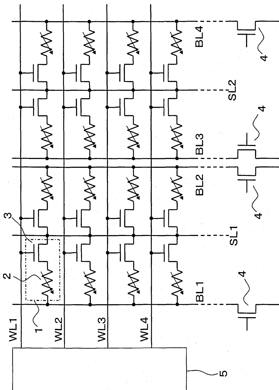
FIG.7 PRIOR ART
