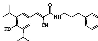
SU1498
