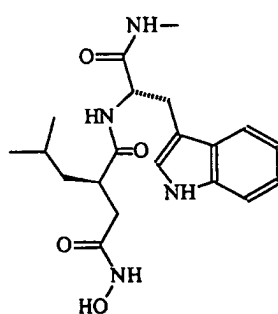
Galardin (Glycomed)
