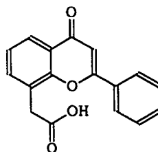
Mitoflaxone (lipha)
