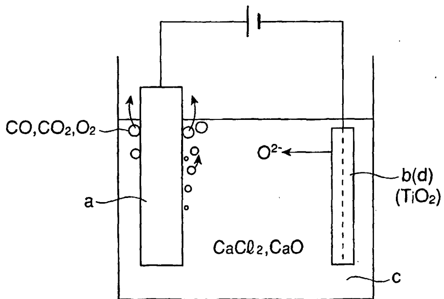
Fig.15 (Prior Art)
