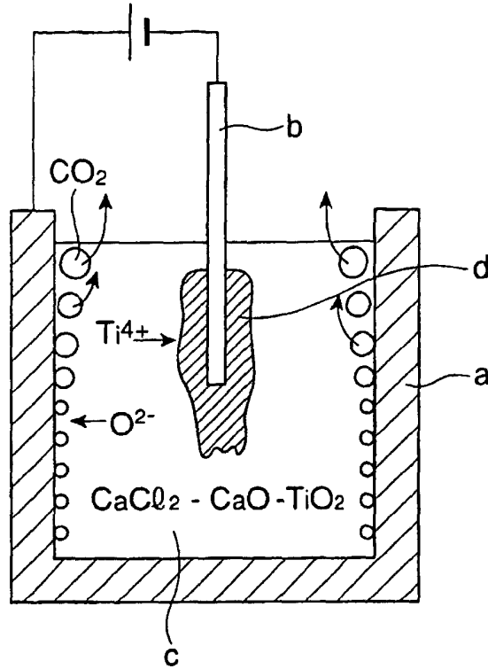
Fig.14 (Prior Art)
