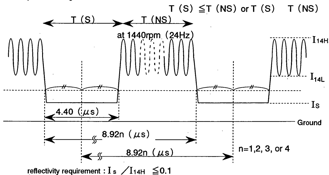
(a) reproduction signal waveform
