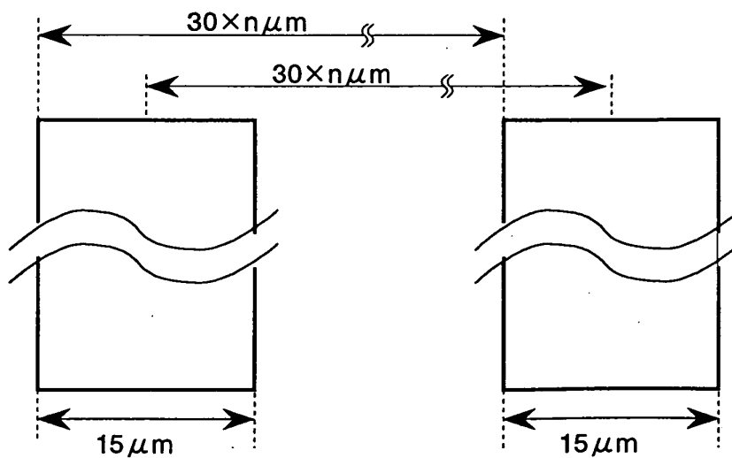
(b) processing precision of slits ( at r=22.2\text{mm} )
