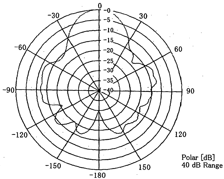
plane \phi = 0^\circ FIG. 47
