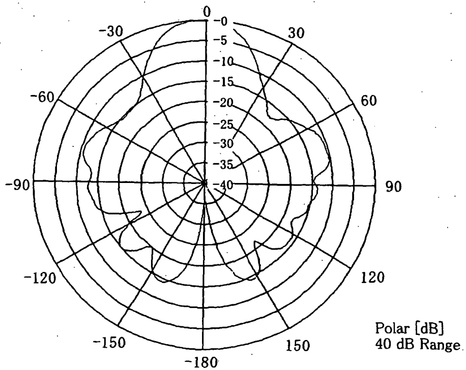
plane \phi = 90^\circ FIG. 48
