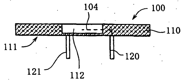
cross-section along the line B-B
