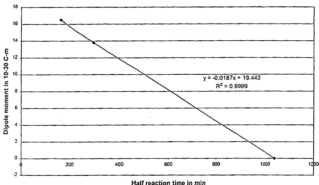
Half-reaction time of the Cyclization Reaction ( Open Form - Toco)
