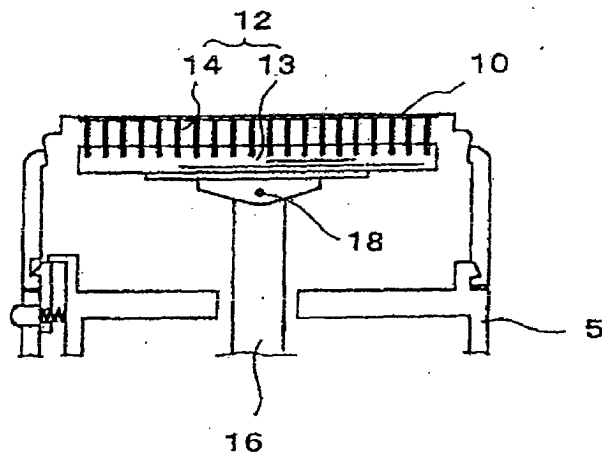
FIG. 9(b) PRIOR ART
