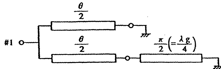
FIG. 24C EQUIVALENT CIRCUIT OF CIRCUIT SHOWN IN FIG. 24A
