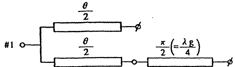
FIG. 24A WHEN PLANE B-B' IS OPEN
