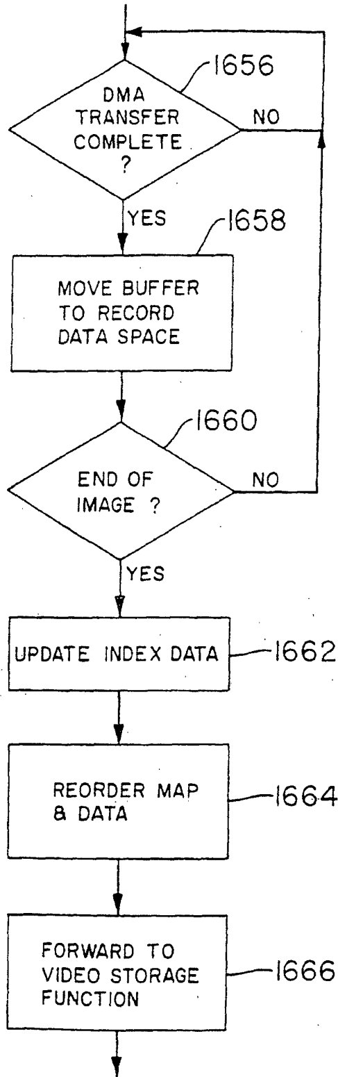
FIG. 71 COMPRESSOR MGR. (VIDEO DATA HANDLING)
