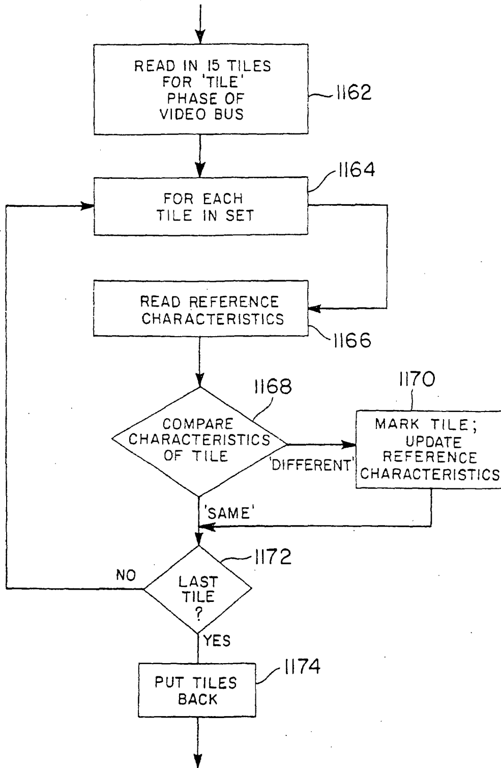
FIG. 42 TILE COMPARING
