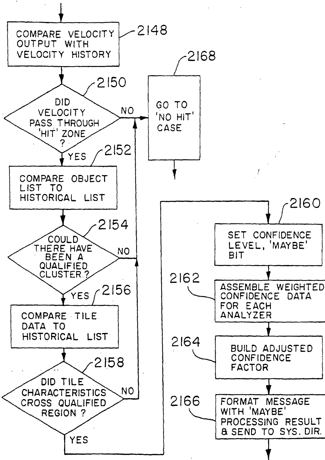
FIG. 95C PROCESSING THE 'MAYBE' CASE
