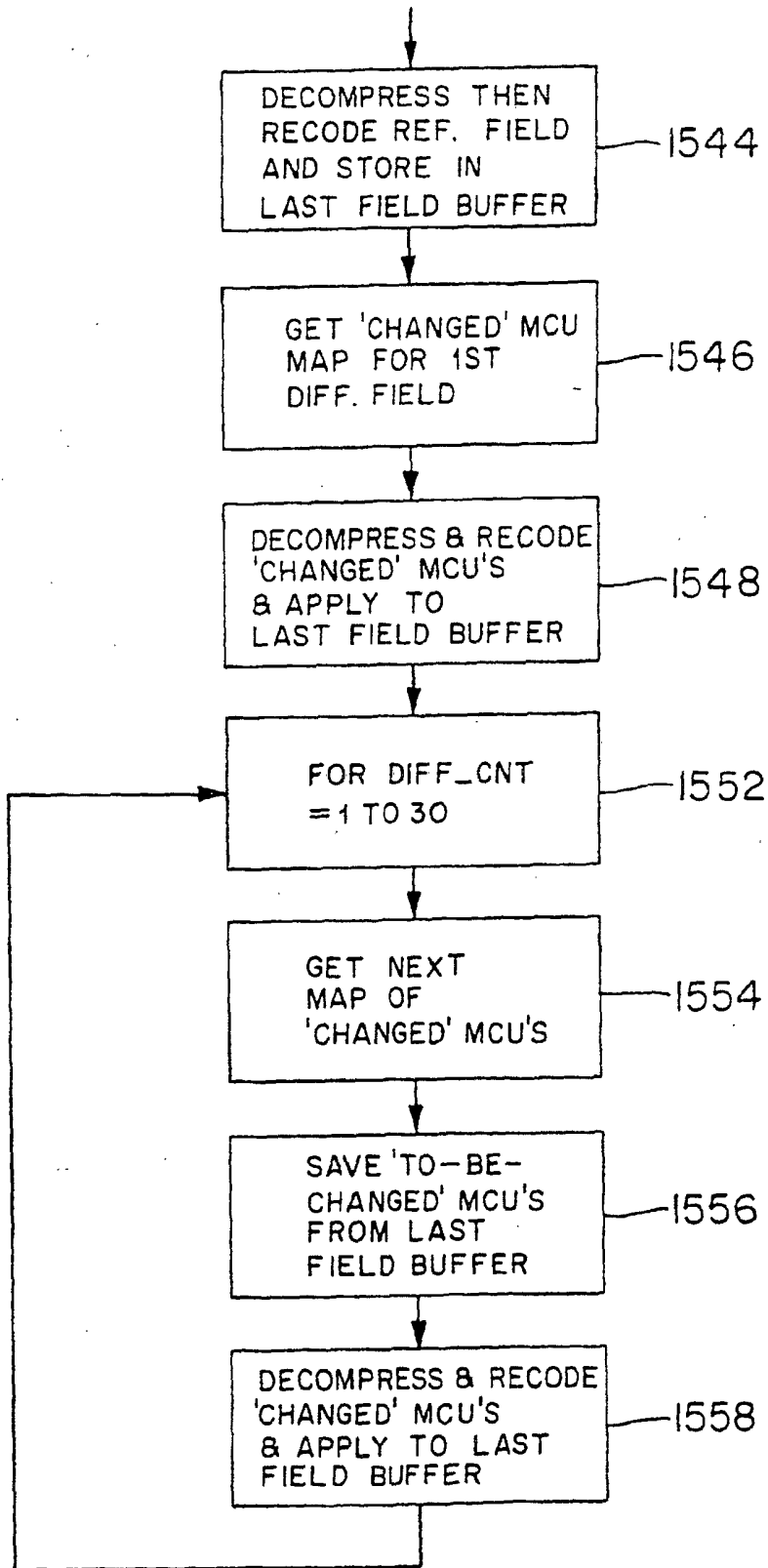
FIG. 66 BUILD BACKWARD HISTORY BUFFER
