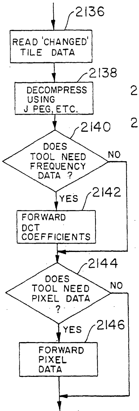
FIG. 95B FEED 'CHANGED' TILE DATA
