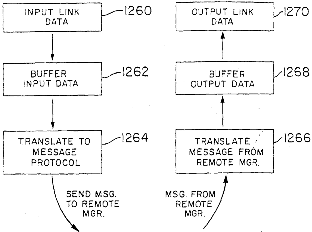
FIG. 48 REMOTE OBJECT INSTANCE
