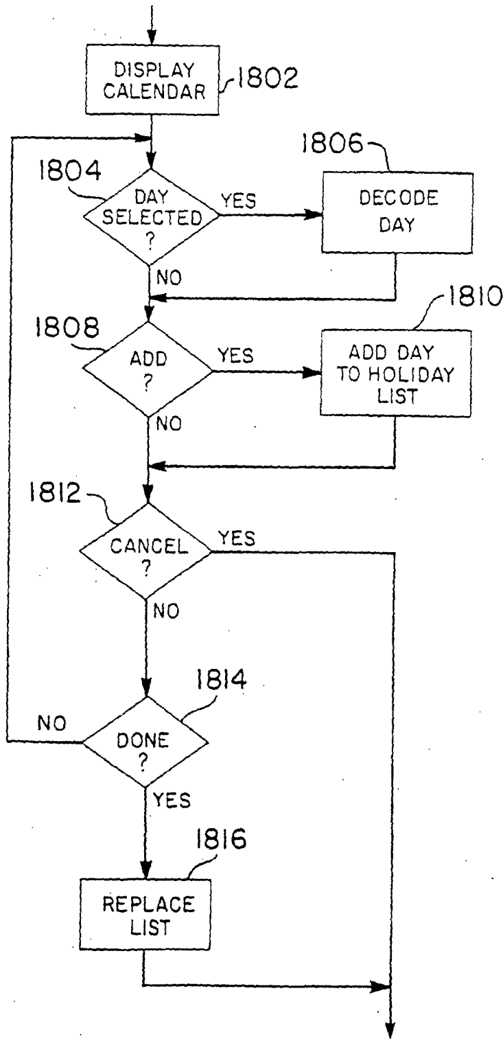
FIG. 80 SCHEDULING: HOLIDAY SETUP
