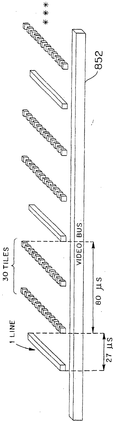
FIG. 26 FULL FIELD MODE: LINES - 30 FIELDS/SEC.; TILES - 240 LINES/2 FIELDS; 3600 TILES/FIELD
