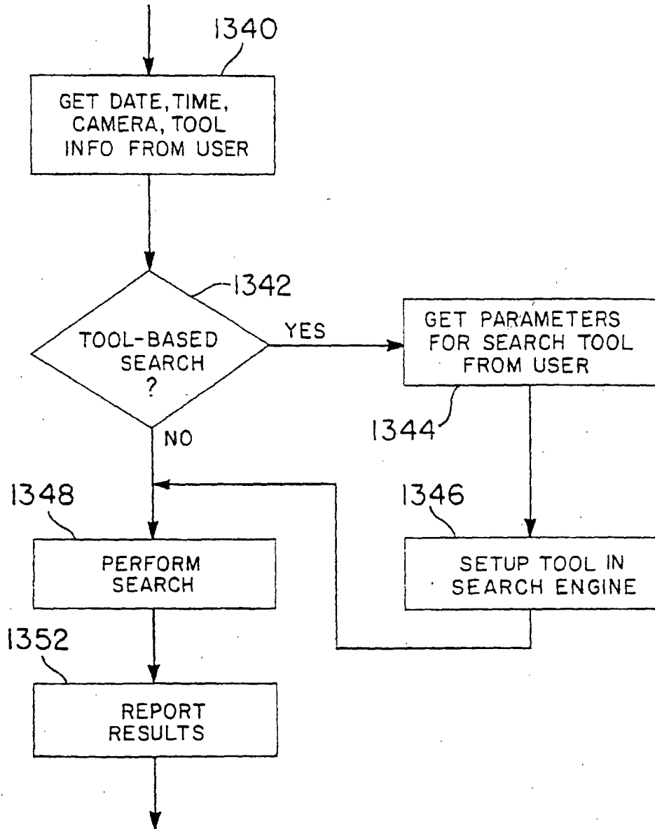
FIG. 53 VIDEO SEARCH
