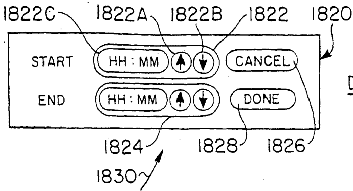
FIG. 85 SCHEDULE QUEUE
