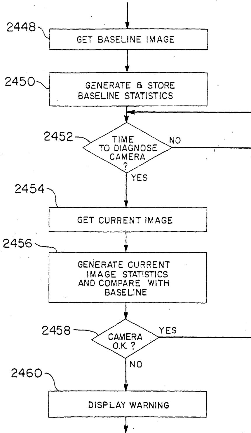
FIG. 120 CAMERA AUTO-DIAGNOSIS
