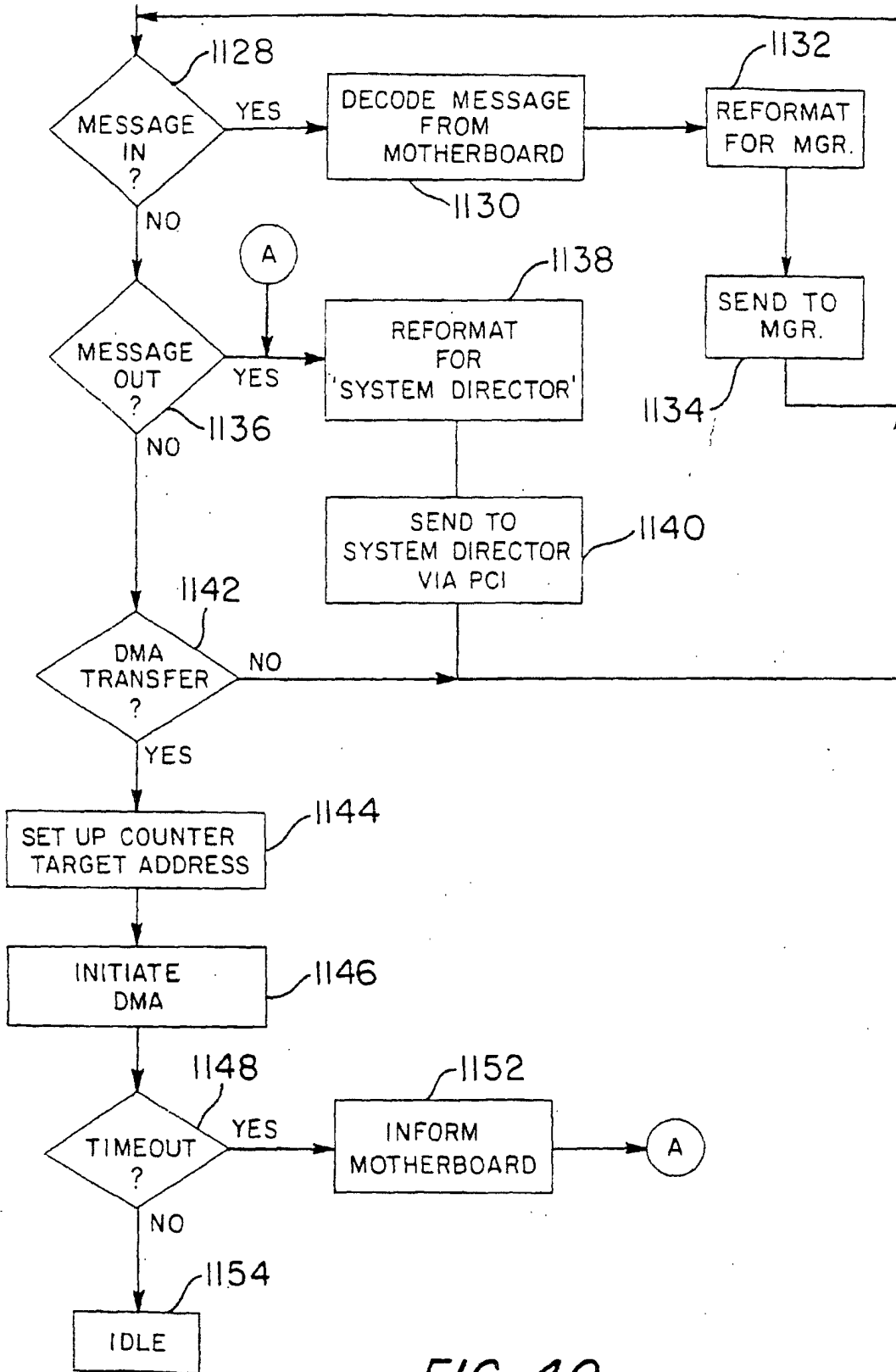
FIG. 40 PCI INTERFACE DRIVER
