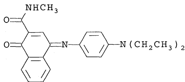
(Cyan Dye 1)
