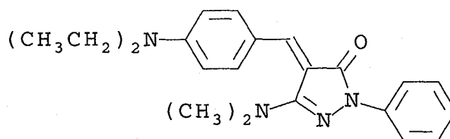
(Yellow Dye 1)
