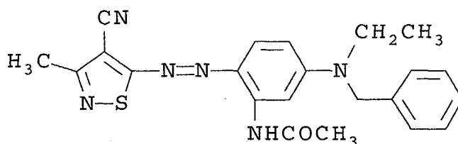
(Magenta Dye 1)
