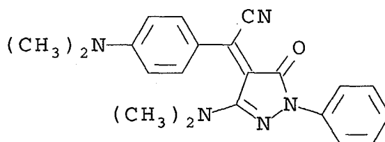
(Magenta Dye 2)
