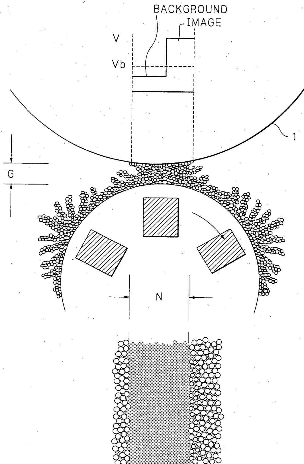
Fig. 1 PRIOR ART
