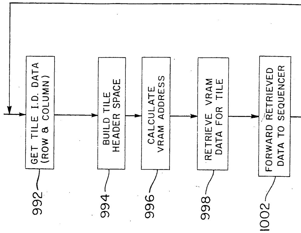
FIG. 33 TILE BUILD LOGIC
