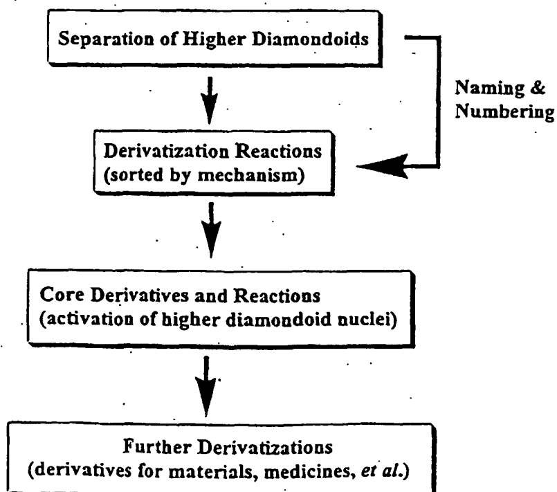
Flow Chart: Strategy for the Derivatization of Higher Diamondoids
