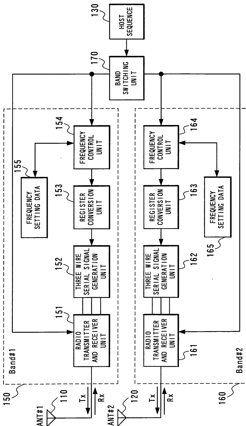
FIG. 5 (PRIOR ART)
