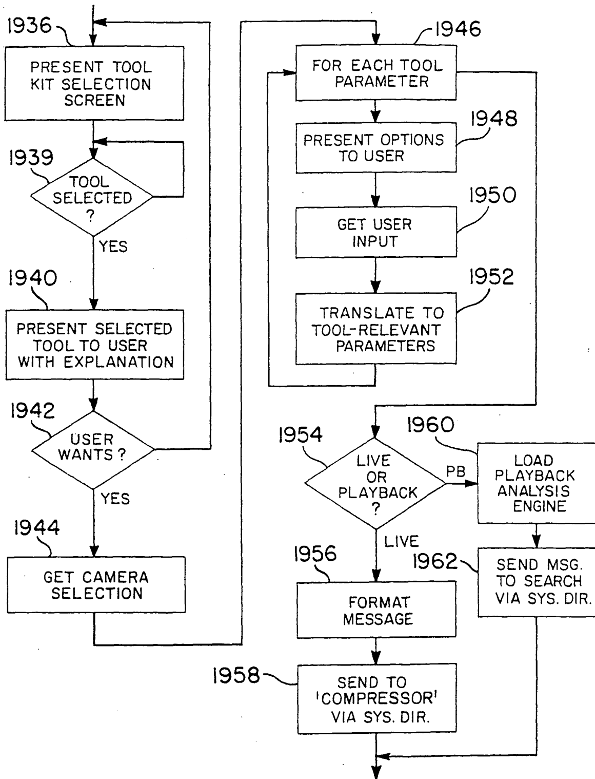
FIG. 89 SELECT & SETUP ANALYSIS TOOL
