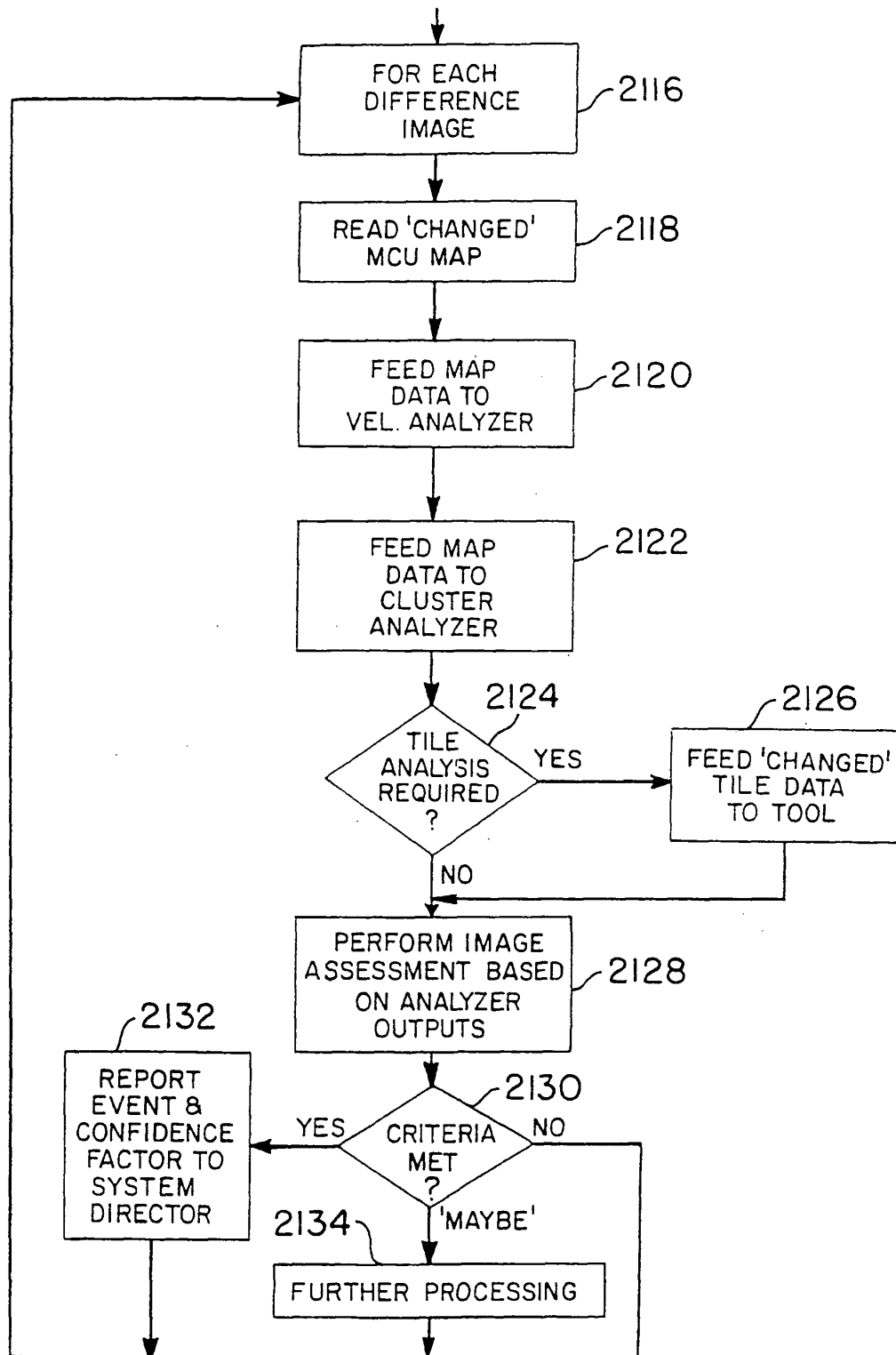
FIG. 95A PLAYBACK ANALYSIS OPERATION
