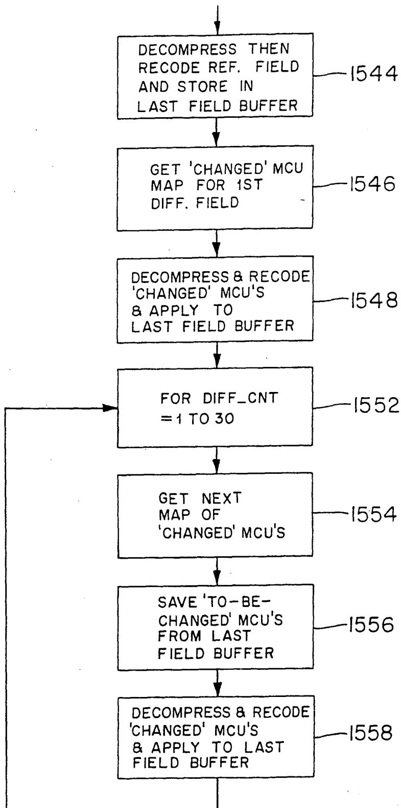
FIG. 66 BUILD BACKWARD HISTORY BUFFER
