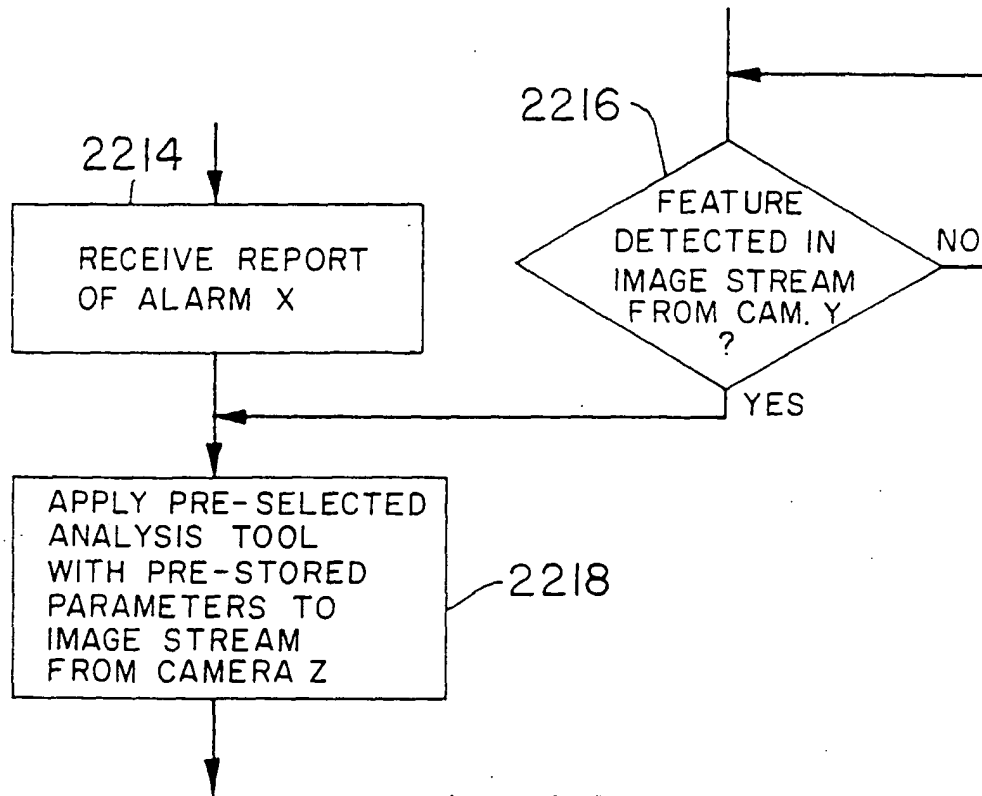
FIG. 98 EVENT-ACTUATED LIVE ANALYSIS TOOL
