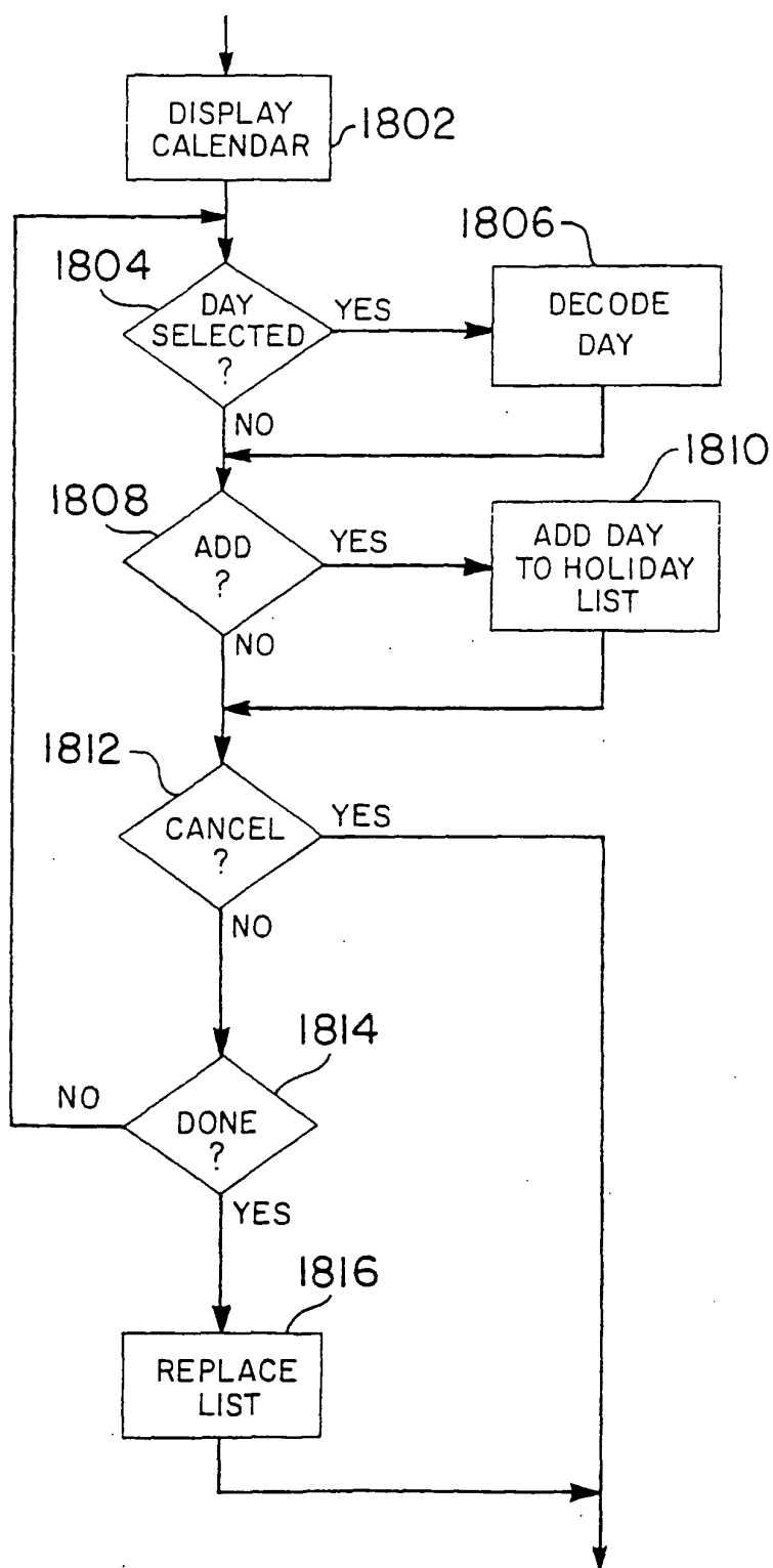
FIG. 80 SCHEDULING: HOLIDAY SETUP
