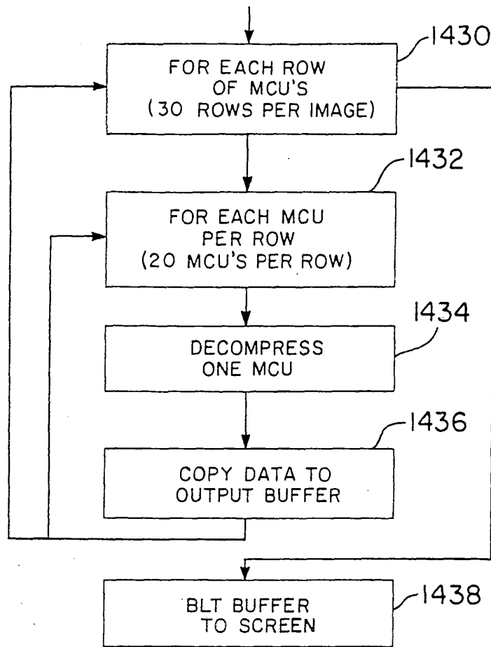
FIG. 57 DECOMPRESS REFERENCE IMAGE
