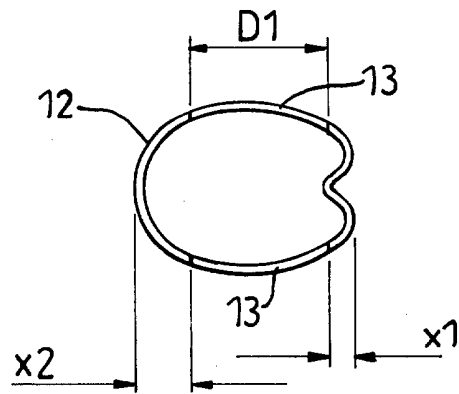
Fig. 9 (PRIOR ART)
