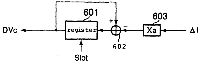
Fig. 3 (Prior Art)
