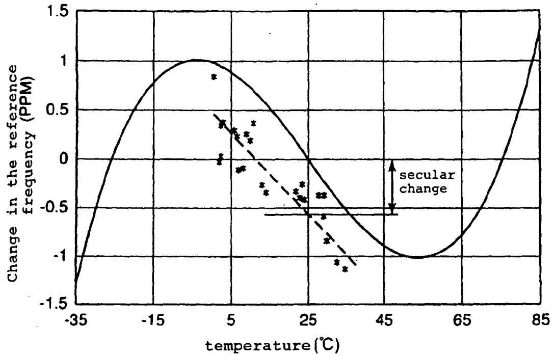
Fig. 5 (Prior Art)
