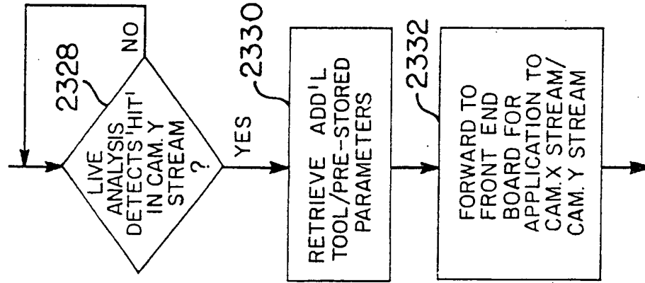
FIG. 106 SOFT-ALARM - ACTUATED LIVE ANALYSIS
