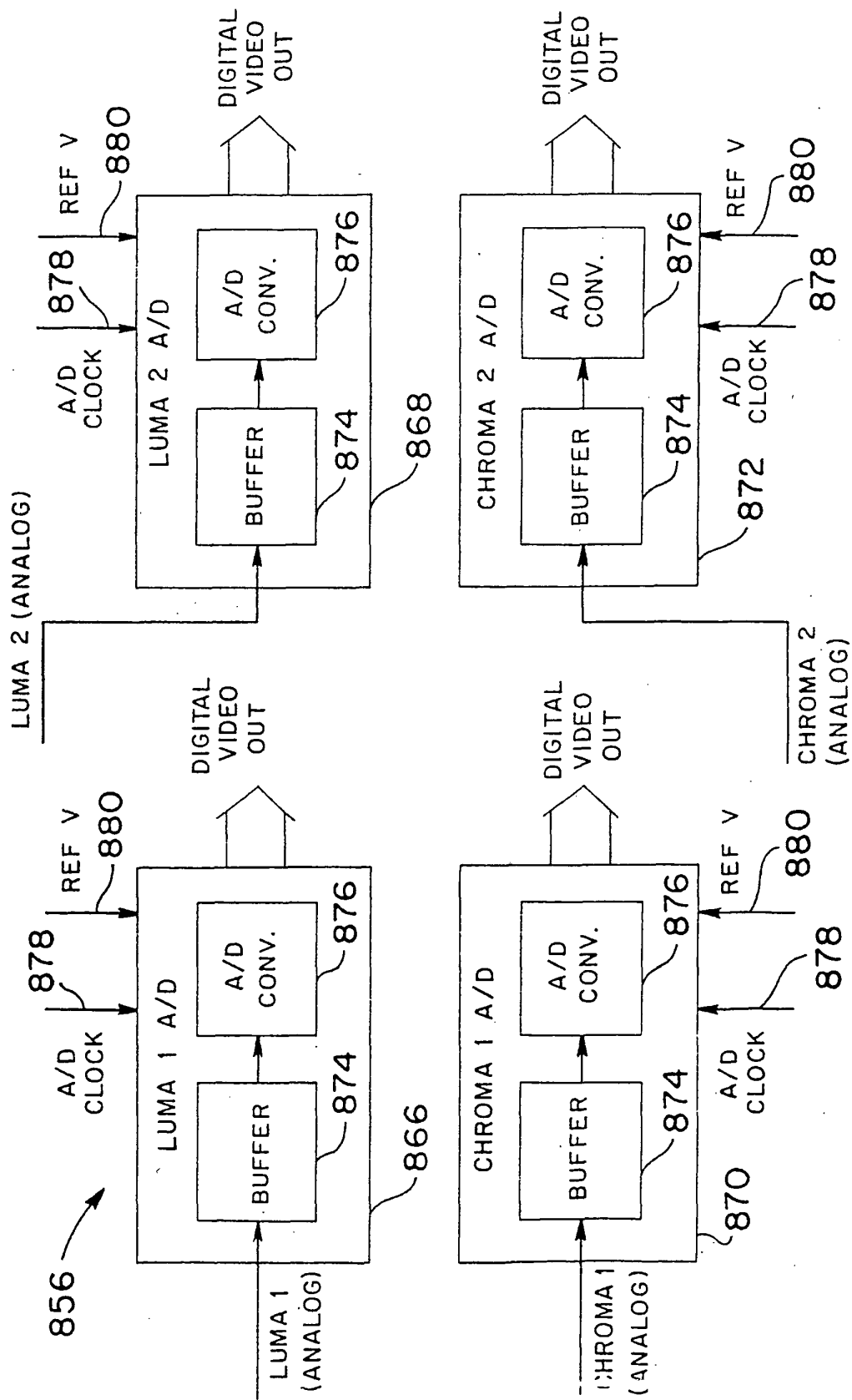
FIG. 16 A/D CONVERSION
