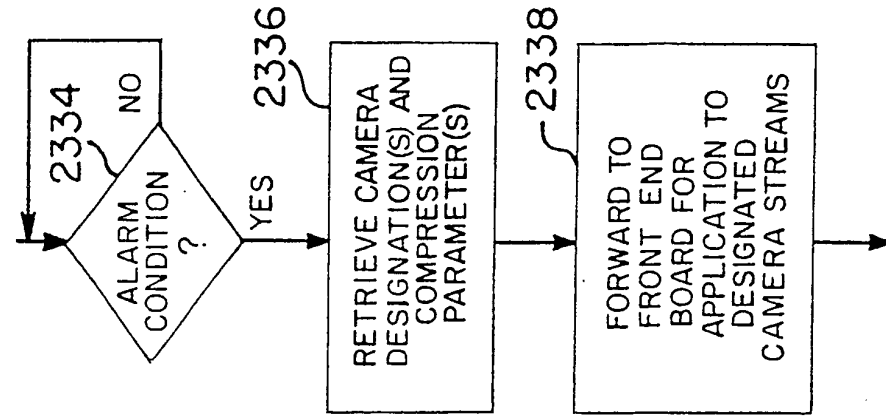
FIG. 107 ALARM - ACTUATED CHANGE IN COMPRESSION
