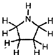
Structural formula (2):
