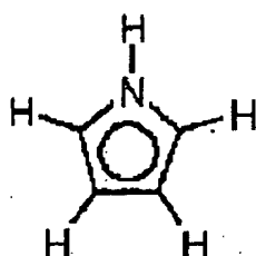
Structural formula (1):
