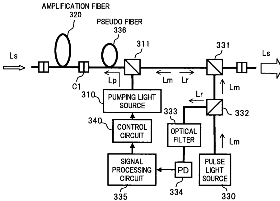
CONFIGURATION OF EMBODIMENT 3-1 OF PRESENT INVENTION
