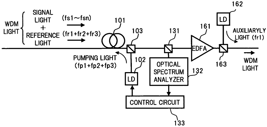
BLOCK DIAGRAM OF REPEATER STATION OF OPTICAL TRANSMISSION SYSTEM ACCORDING TO EMBODIMENT 1-2
