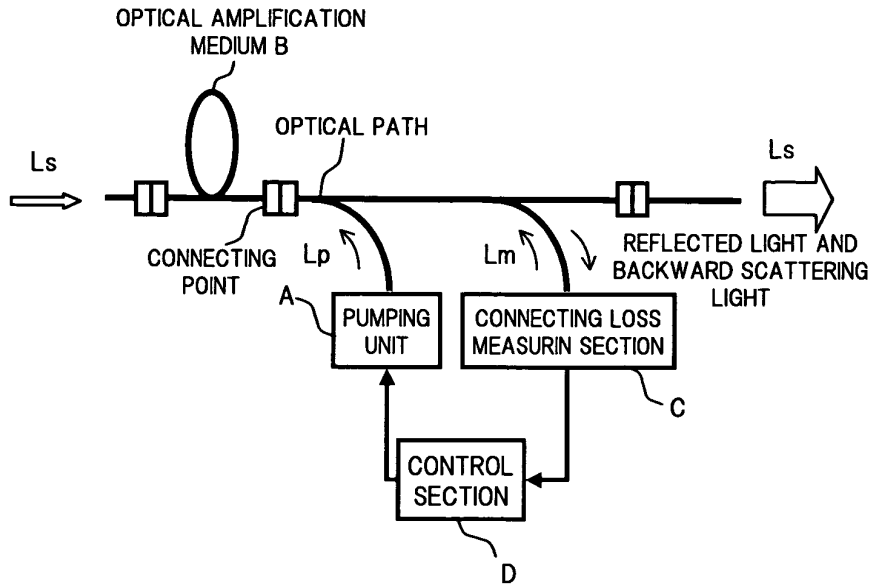
BASIC CONFIGURATION OF EMBODIMENT 3 OF PRESENT INVENTION
