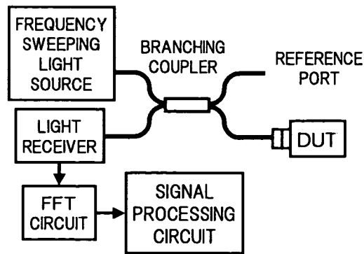
TYPICAL OFDR MEASURING SYSTEM
