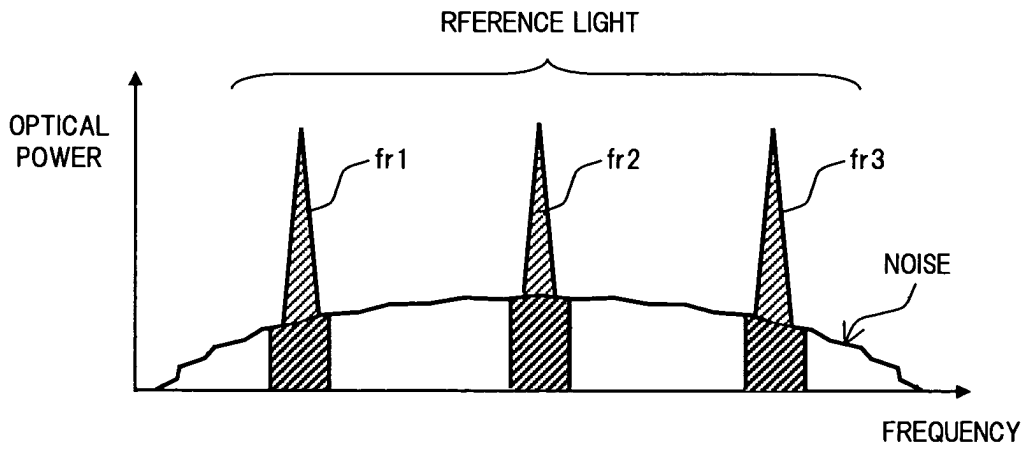
DIAGRAM EXPLAINING OPTICAL DETECTION IN EMBODIMENT 1-1
