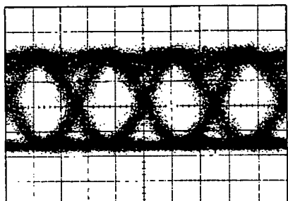
(a) 40Gb/s NRZ MODULATED SIGNAL LIGHT
