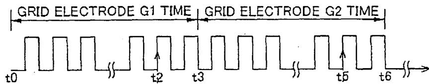
(B) INTERNAL CLOCK SIGNAL A
