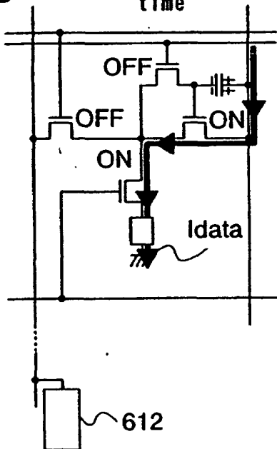
Fig. 17C light emitting time
