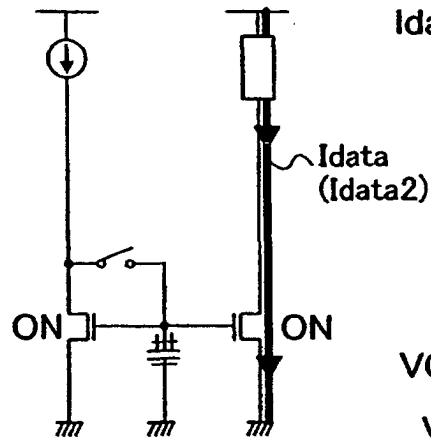
Fig. 20C signal input time to pixel
