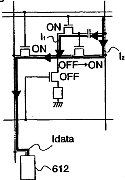
Fig. 17A signal input time
