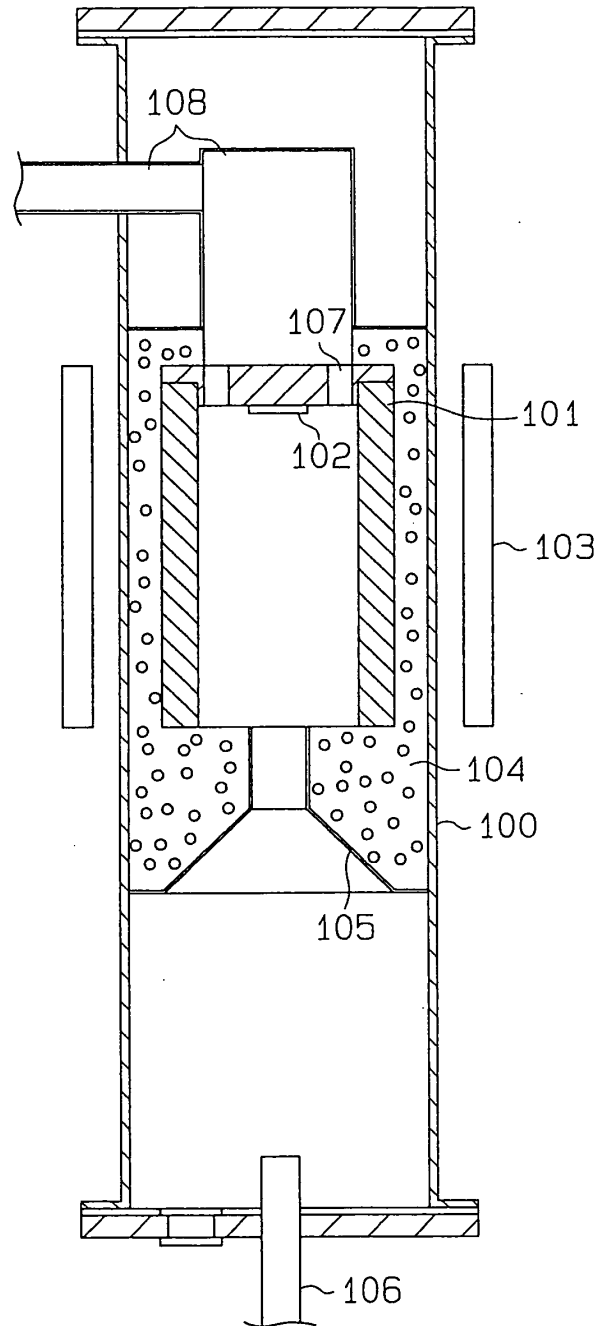
FIG. 20 PRIOR ART
