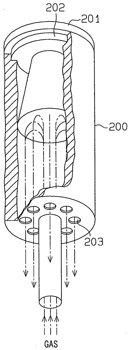
FIG. 21 PRIOR ART
