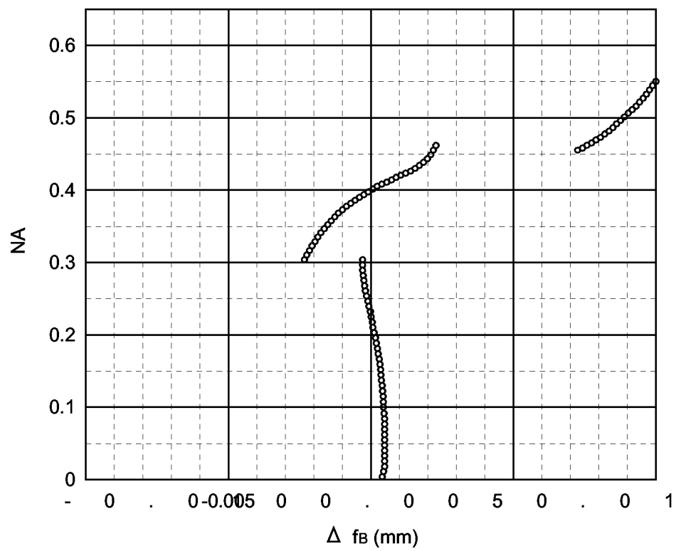
CD LONGITUDINAL SPHERICAL ABERRATION DIAGRAM
