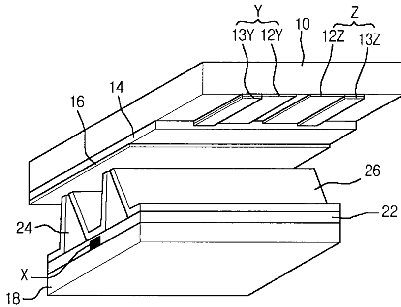
Fig.2 Related Art
