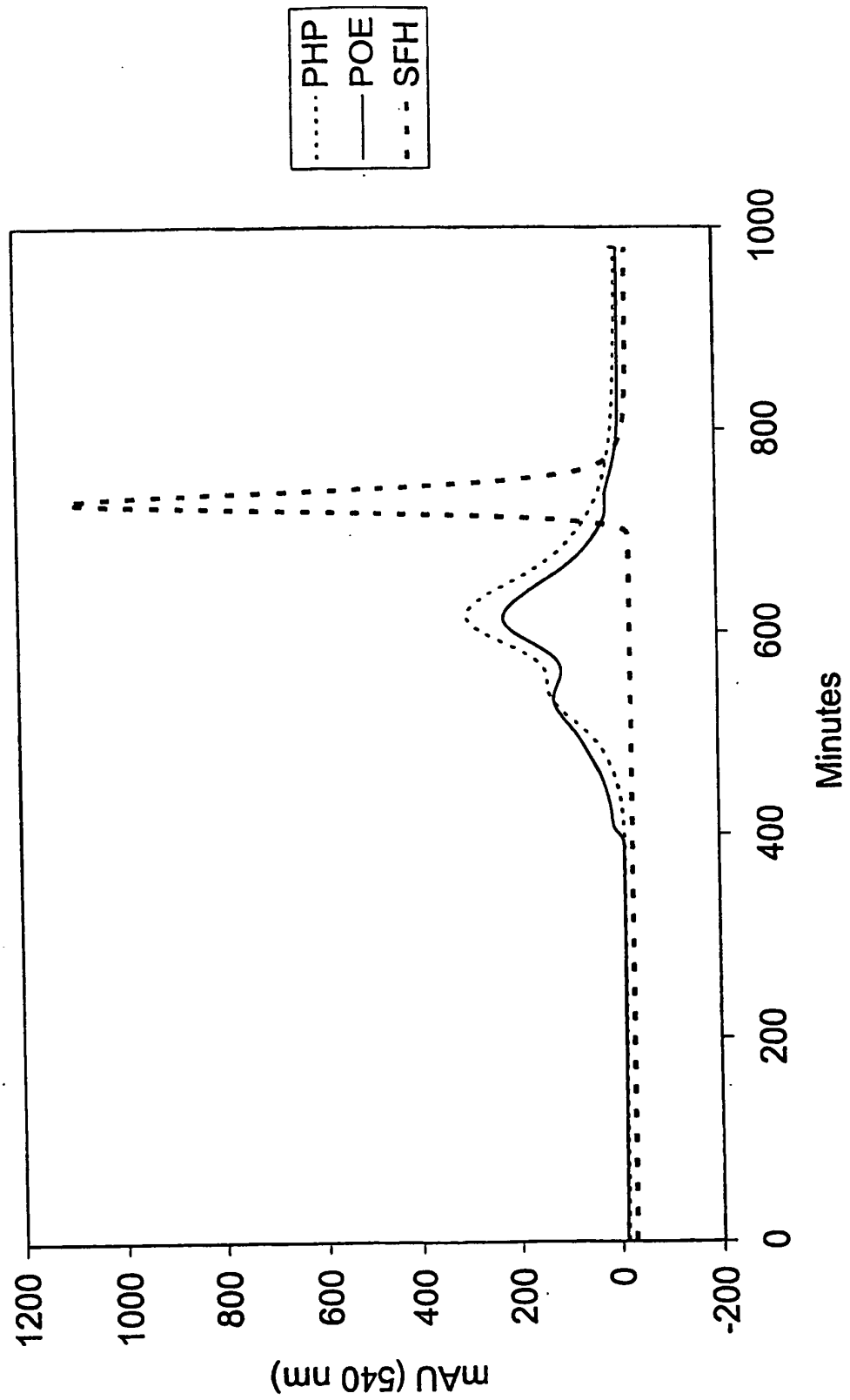
Figure 3 Size Exclusion Chromatography
