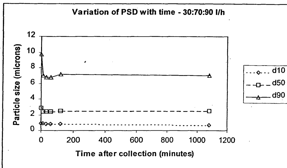
Figure 7: Variation in Particle size with time for 30:70:90 I/h suspension
