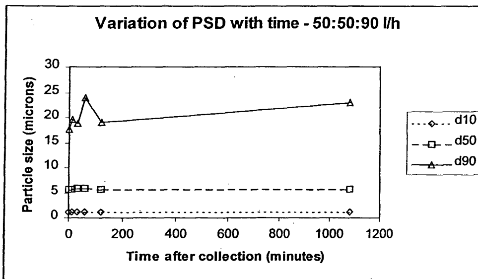
Figure 8: Variation in Particle size with time for 50:50:90 I/h suspension
