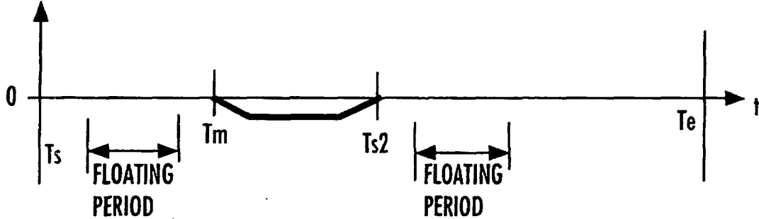
FIG.26 BODY INCLINATION RESTORING MOMENT ZMP-CONVERTED VALUE (ZMP prec )
