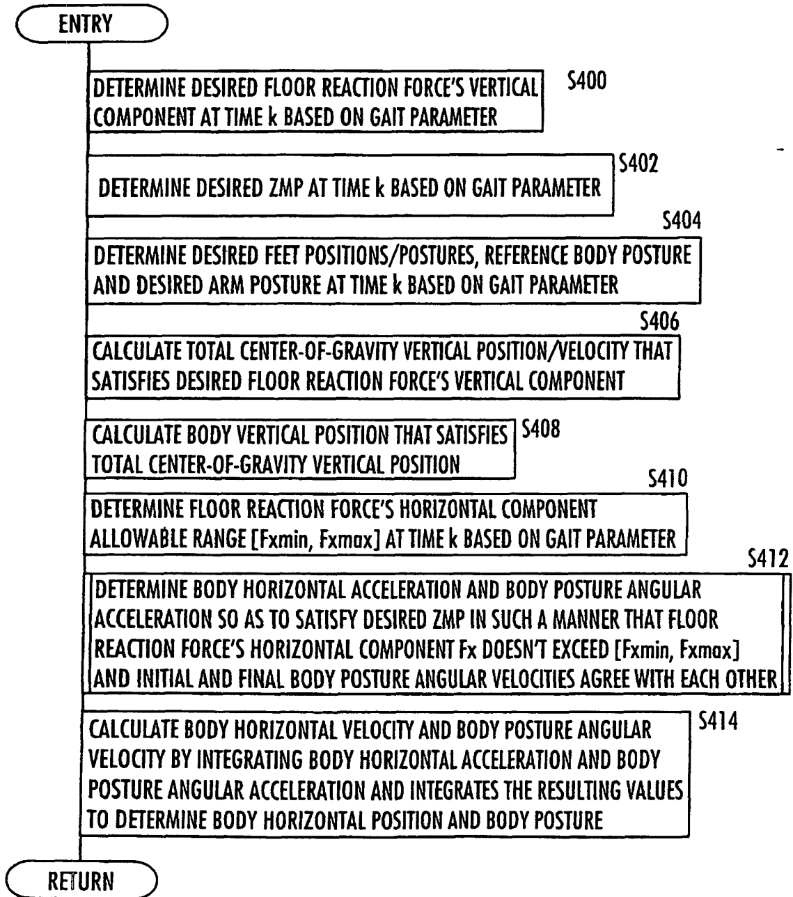
FIG.21 ( PROCESS OF DETERMINING NORMAL GAIT INSTANTANEOUS VALUE )
