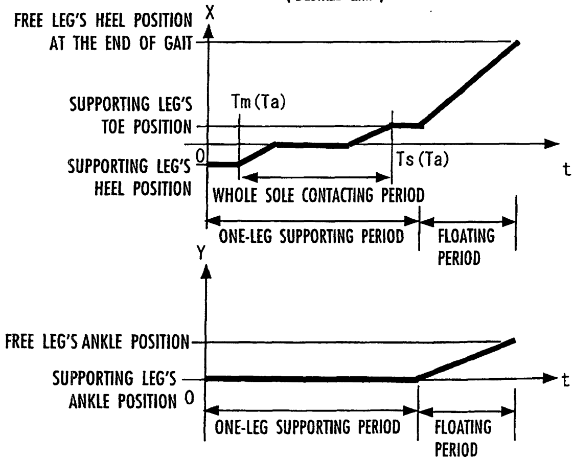
FIG.7 ( DESIRED ZMP )
