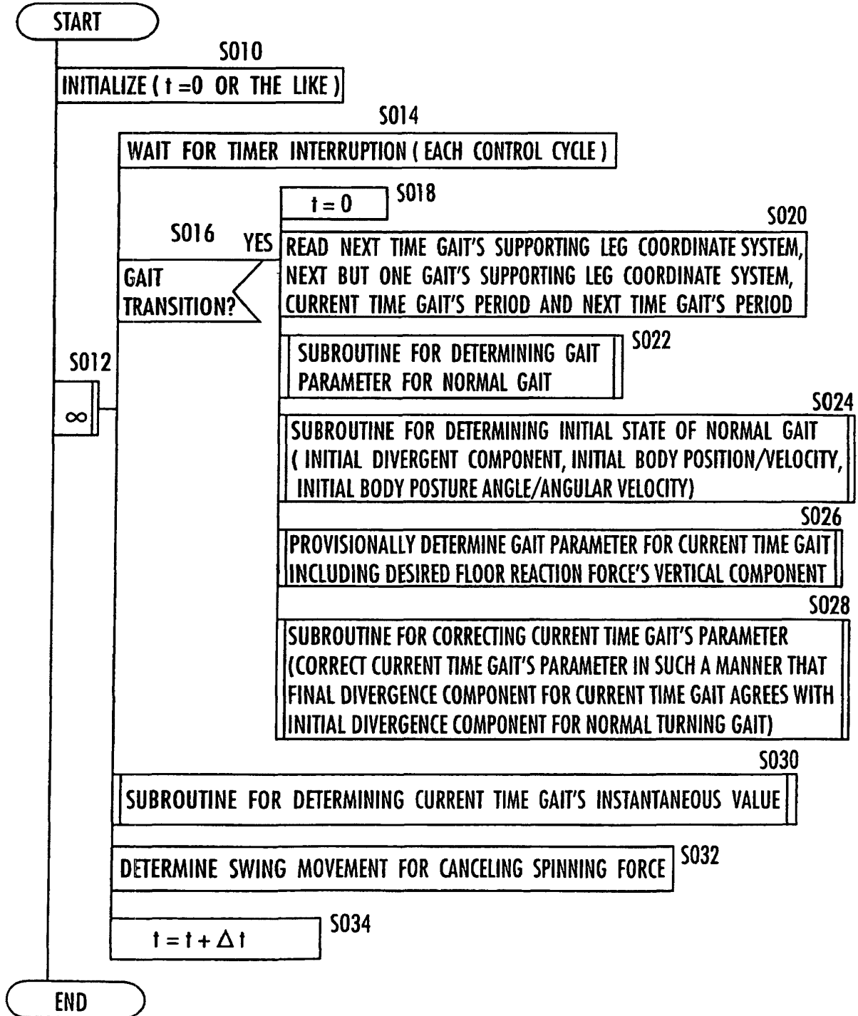
FIG.12 ( FLOWCHART OF GAIT GENERATION PROCESS )
