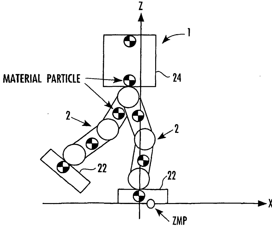
FIG.11 ( FULL MODEL )
