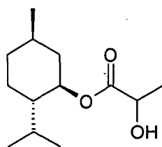
l-menthyl lactate
