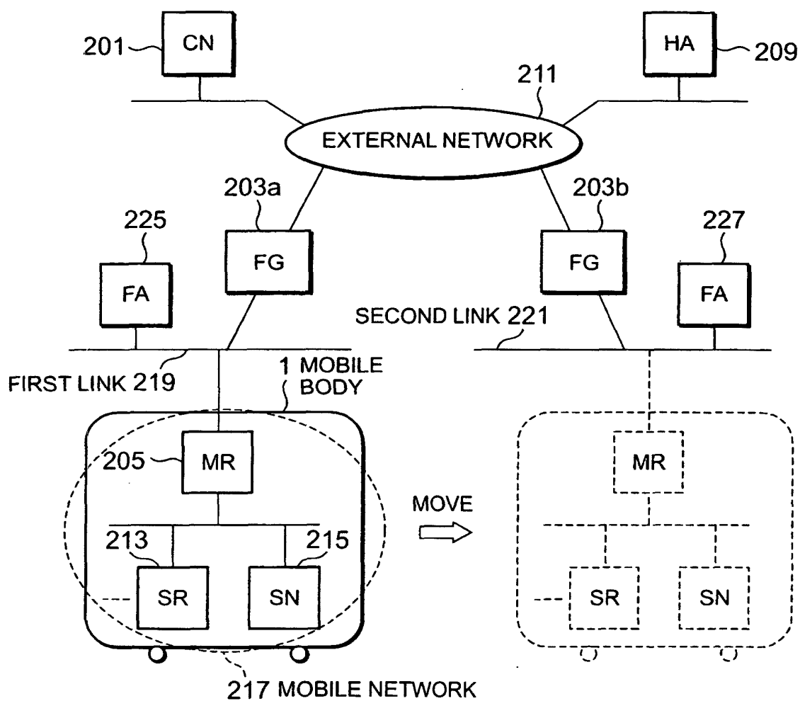
FIG. 12 PRIOR ART
