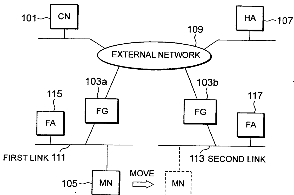
FIG. 11 PRIOR ART
